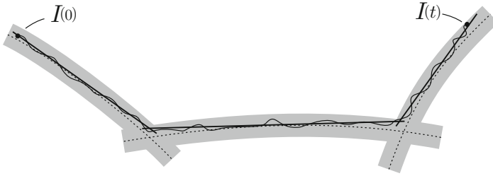
Fig. 1. Illustrating the possible mechanism of fast diffusion through crossing of fast drift planes, if resonances are not well separated. Dashed curves the resonant manifolds. Gray neighbours the corresponding resonant regions. Lines : the planes of fast drift. Irregular curve a possible motion of actions from I(0) to I(t) , in a time of order 1/\epsilon
