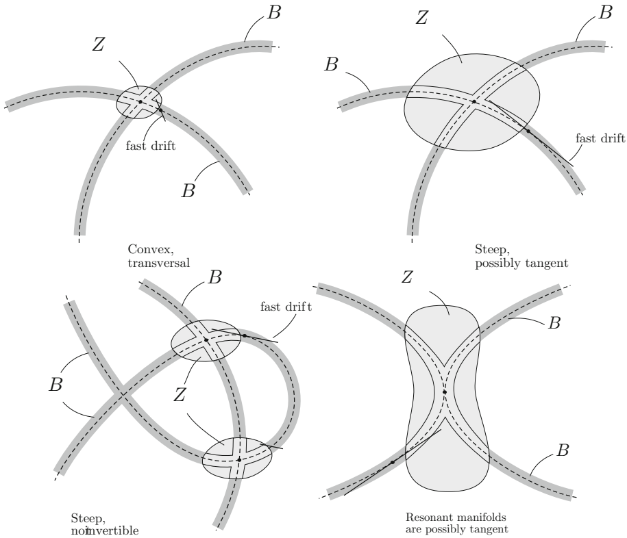
Fig. 2. Sketch of the resonant sets: two resonances related to the lattices \Lambda and \Lambda' of the same multiplicity j are sketched, together with the resonance related to the lattice \Lambda \oplus \Lambda' of multiplicity j + 1 , identified at the crossing of the two previous resonances, and some fast drift lines. Precisely, dashed curves represent the resonant manifolds of multiplicity j ; dark gray areas denote resonant blocks of multiplicity j ; light gray areas represent resonant zones of multiplicity j + 1 ; by \lambda we denote some j dimensional fast-drift lines. Different situations are illustrated: in the top-left panel we plot the situation which is typical of the quasi-convex cases, with the fast drift planes which are transverse to the resonance; in the other panels we illustrate some situations which one may encounter in the more generic steep cases, where the fast drift planes may be tangent to the resonant manifolds, and also self-intersections ( bottom-left panel ) and tangencies of resonances ( bottom-right panel ) are possible. In all the represented cases, the fast drift lines \lambda = (I + \langle \Lambda \rangle) \cap \mathcal{Z}_\Lambda or \lambda = (I + \langle \Lambda' \rangle) \cap \mathcal{Z}'_{\Lambda'} through points I \in B_{\Lambda \oplus \Lambda'} do not intersect other resonant blocks of multiplicity j + 1
