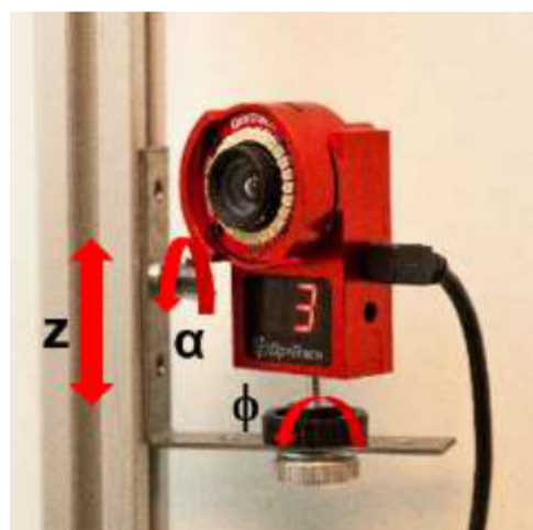
Figure 5 Fix system of the camera that allow the rotation in two directions
