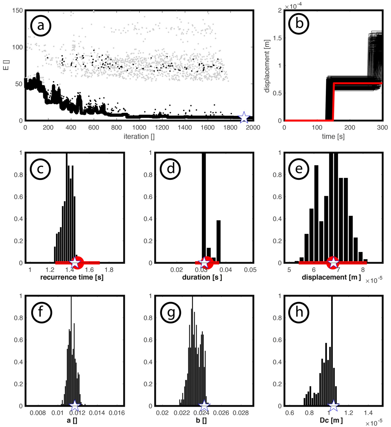
Figure 4. Simulated annealing method and route toward the preferred rate and state parameters combination. (a) Evolution of the error E during the parameter search. The black solid line in panel a highlights the path of accepted simulations. Successful simulations that fall within Foamquake's Me \pm SD/2 are highlighted by black dots and reported in the following panels. Panels (b) shows displacement-time curve for successful numerical simulations (black) compared against Foamquake median (red) distribution of model parameters (panel c–e) and distribution of rate and state parameters (panels f–h) for successful simulations. Red circles and horizontal lines in panels (c–e) represent Foamquake's Me \pm SD/2 . White stars represent the simulation with lowest error. A line-time representation of this model is reported in Figures 8a and 8b.
