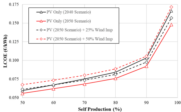
Fig. 13. LCOE comparison: only PV (2040 and 2050 cost scenario) and PV+wind import (25 and 50 %) as function of self-production.
