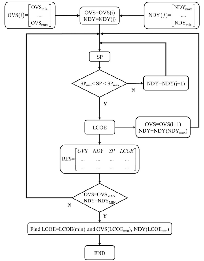
Fig. 1. Block diagram of the minimization process.
