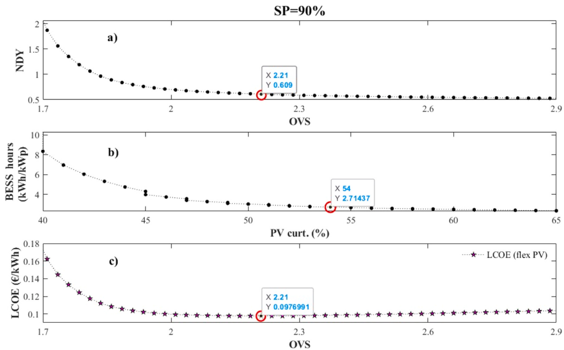
Fig. 10. Simulation results for SP = 90 % showing trends of NDY, LCOE as a function of oversize and BESS hours as function of PV curtailment with 25 % wind import.
