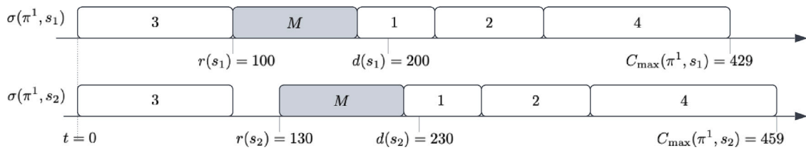
Fig. 1. The realization schedules \sigma(\pi^1, s_1) and \sigma(\pi^1, s_2) of the sequence \pi^1 = \langle 3, 1, 2, 4 \rangle under the two scenarios of Example 1.
