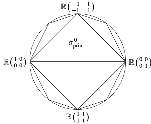
Figure 1: A section of \Omega_2^{\text{tr}} and its perfect cone decomposition.
