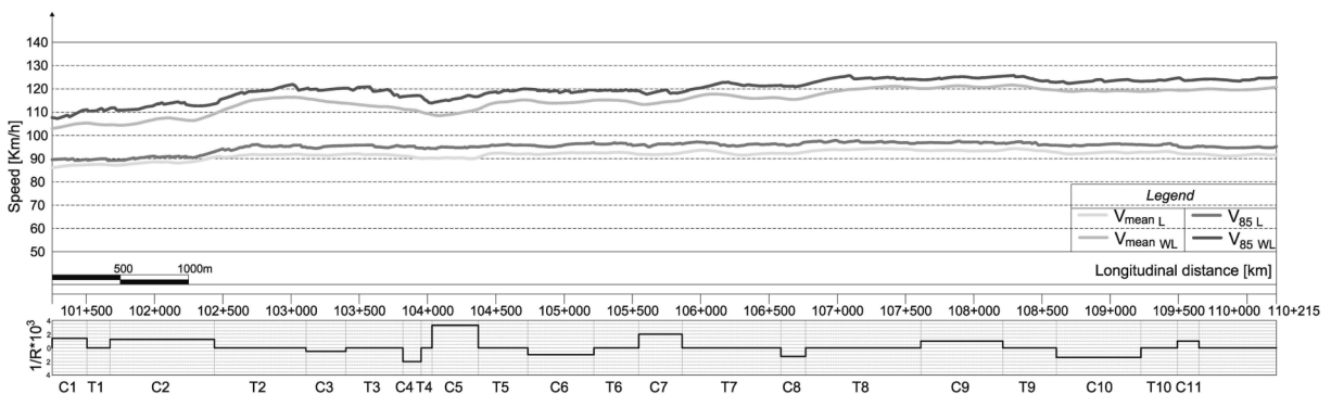
Fig. 6. Mean and operating speed profiles of drivers' sample in configurations with ( V_{\text{mean L}} and V_{85 \text{ L}} , respectively) and without ( V_{\text{mean WL}} and V_{85 \text{ WL}} , respectively) posted speed limits on the second motorway's segment.
