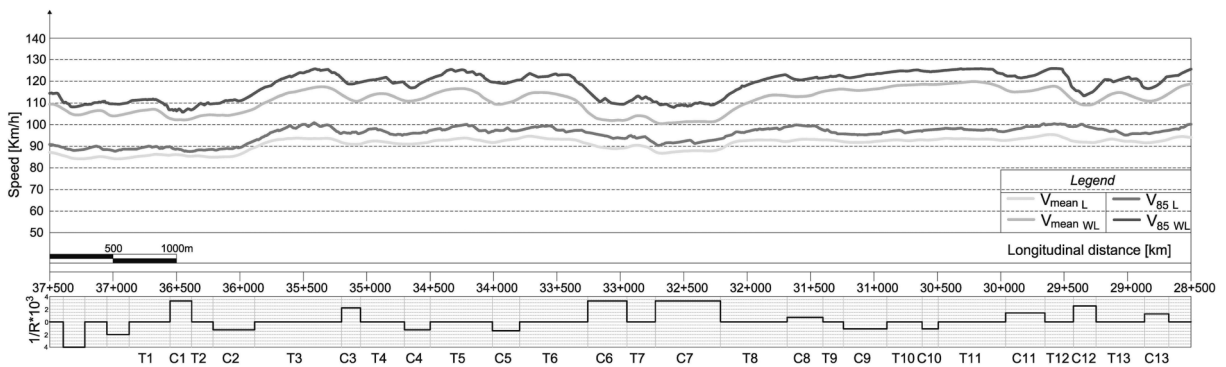
Fig. 5. Mean and operating speed profiles of drivers' sample in configurations with ( V_{\text{mean L}} and V_{85 \text{ L}} , respectively) and without ( V_{\text{mean WL}} and V_{85 \text{ WL}} , respectively) posted speed limits on the first motorway's segment.
