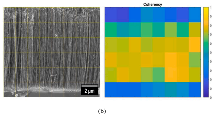
Fig. 3. Side view SEM image (at 25 K magnification) along with corresponding heatmaps representing the coherency values for different ROIs for VA-CNTs grown via (a) thermal CVD and (b) PECVD methods, respectively.
