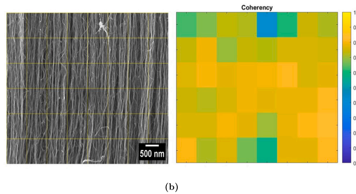
Fig. 4. Side view SEM image (at 50k magnification) along with corresponding heatmaps representing the coherency values for different ROIs for VA-CNTs grown via (a) thermal CVD method (b) PECVD method respectively.
