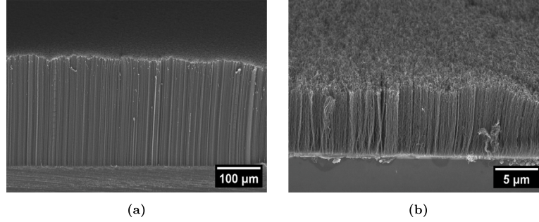
Fig. 2. Side view SEM image of VA-CNTs grown via (a) thermal CVD and (b) PECVD method, respectively.
