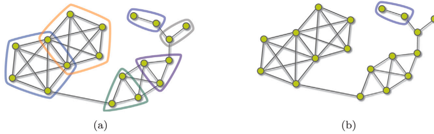
Fig. 9. (a) A c -covering summary S with c = 1 : each vertex of the graph is contained into at least one maximal clique in S . (b) A summary S with all the \ell -isolated maximal cliques when \ell = 1 : the chosen maximal cliques have less than k outgoing edges.
