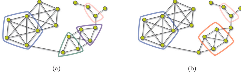
Fig. 8. Examples of internal overlap summarization. (a) A \sigma -independent summary S with \sigma = 0 . (b) A \rho -edge-independent summary S with \rho = 0 .
