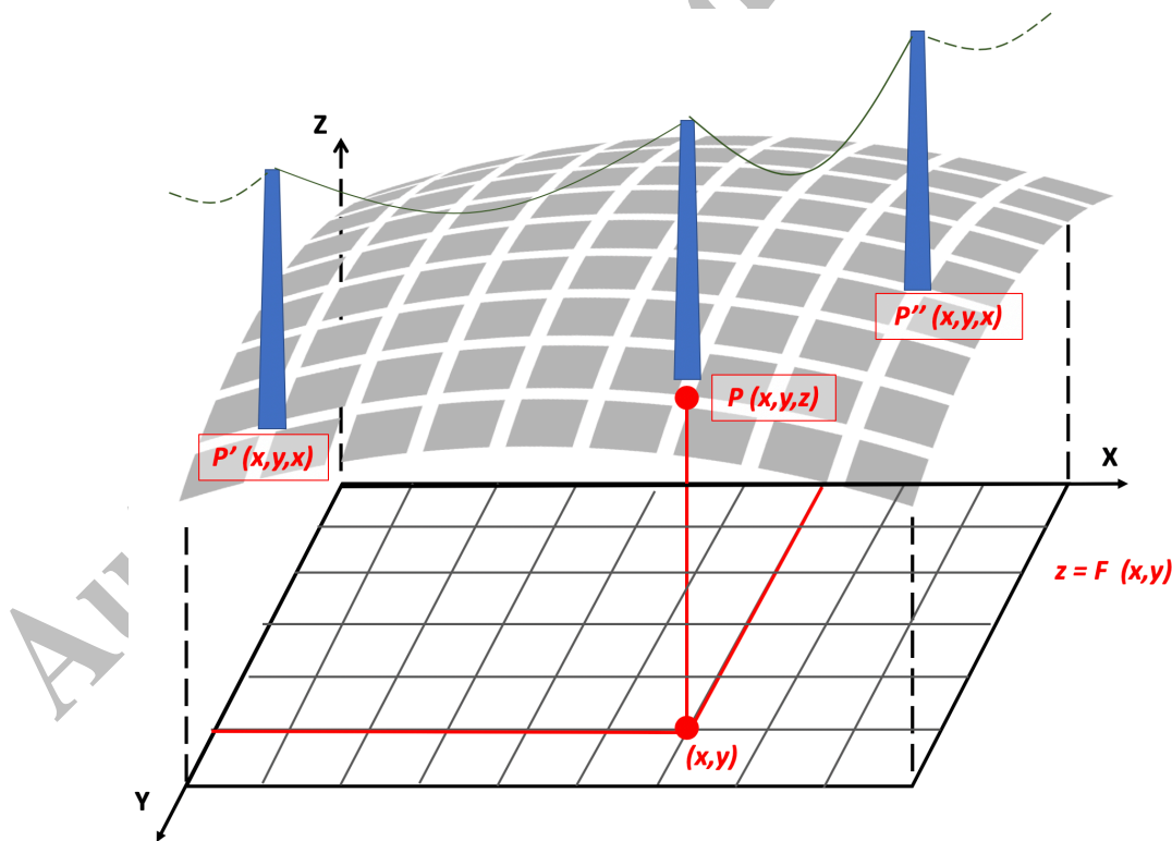
Figure 8: The schematic representation of a simplified line where each pole has a parametric position described by Cartesian coordinates.
