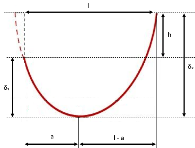
Figure 10: Catenary with uneven supports.
