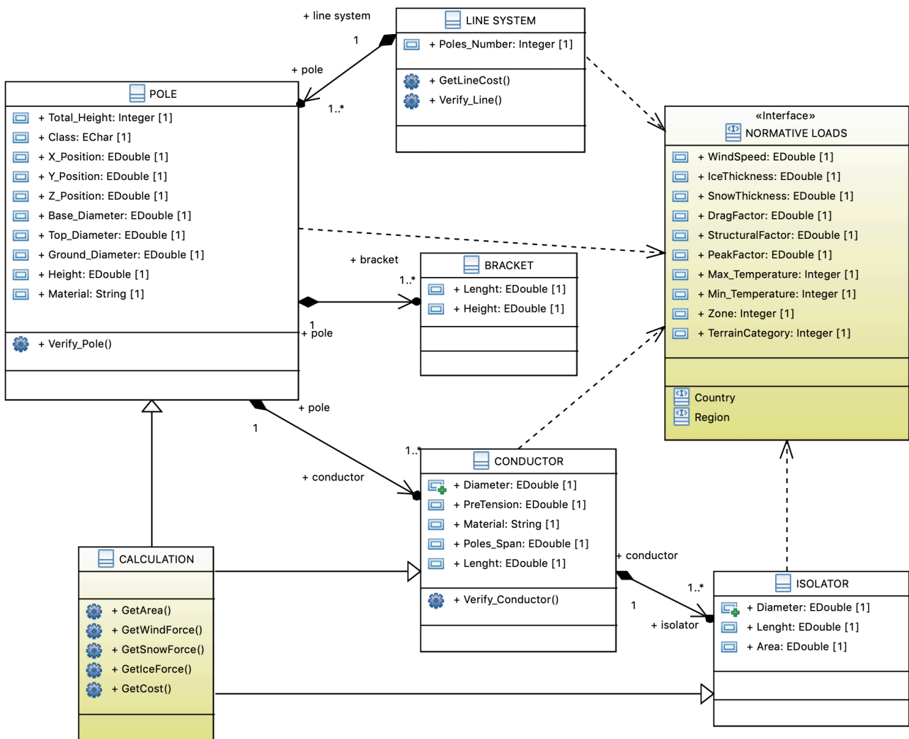
Figure 5: The composite structure diagram related to the analyzed system.
