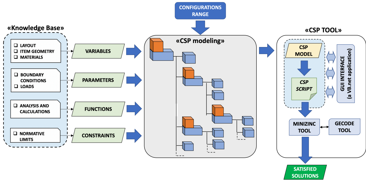
Figure 3: The architecture of the design platform proposed for the CSP analysis and modeling.
