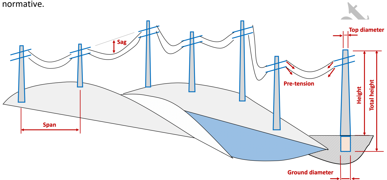
Figure 1: A representation of an overhead electrical line.
