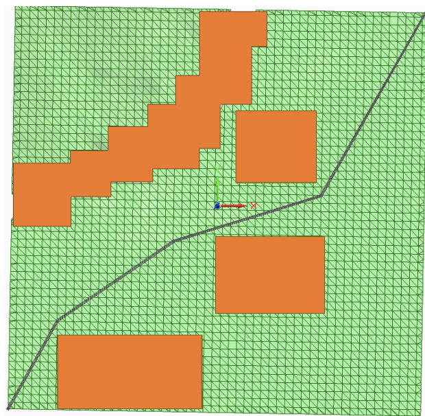
Figure 18: Top view of the 5-pole line with the obstacle areas.
