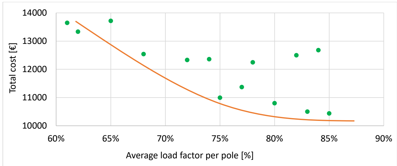
Figure 14: The result of the optimization analysis outlined in the orange line the relative Pareto front (results for 7,56-mm conductors). The cost values are related to poles and conductors.
