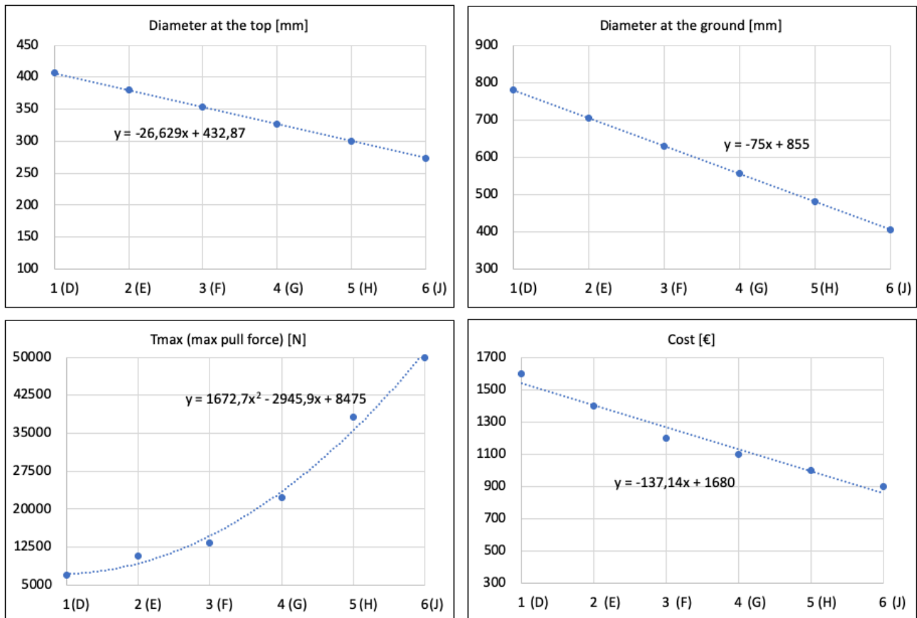
Figure 12: The discretization of the pole’s parameters for a specific height ( H=14 m) in function of each class (D, E, F, G, H, J).
