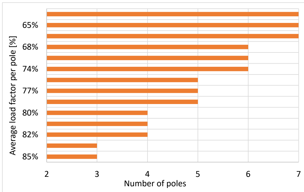
Figure 15: The correlation between the number of poles and the average load factor per pole.
