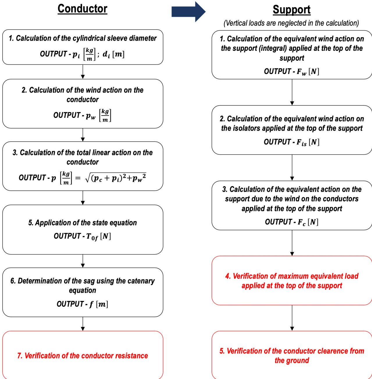
Figure 11: Scheme of the implemented verification process for each loading condition.
