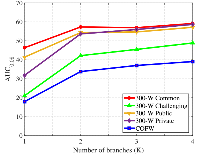
Fig. 13. Ablation study results for the proposed CCNN scheme: performance in terms of AUC_{0.08} when varying the number of cascades in both the CHCNN (heatmap) and CRCNN (regression) subnetworks.
