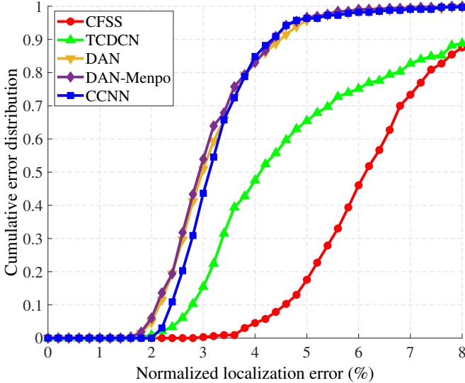
Fig. 6. CEDs vs. NLE results for the HELEN test set.
