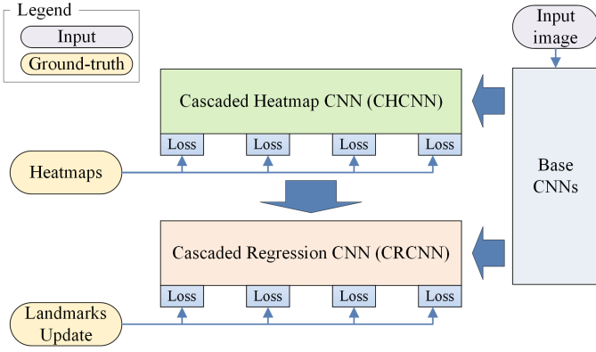
Fig. 2. Outline of the proposed CCNN framework. The CCNN consists of base CNNs, preceding the cascaded heatmap subnetwork (CHCNN) estimating the heatmaps, and the cascaded regression CNN (CRCNN) refining the heatmaps localization via point-wise regression.
