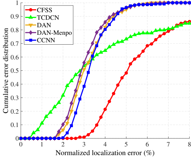
Fig. 5. CEDs vs. NLE results for the LFPW test set.
