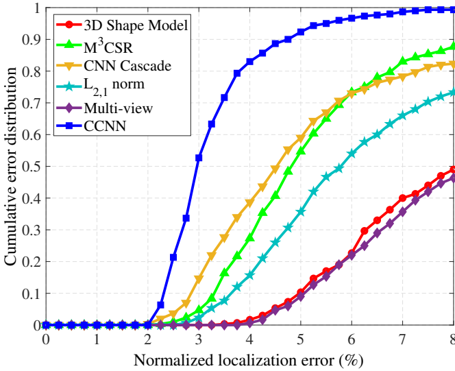
Fig. 8. CEDs vs. NLE results for the 300-W outdoor test set.
