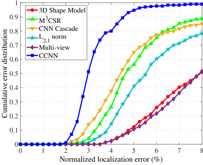
Fig. 7. CEDs vs. NLE results for the 300-W indoor test set.
