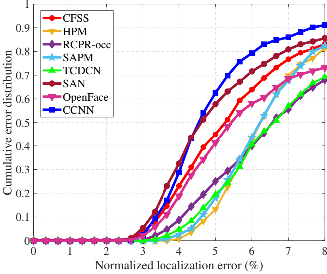
Fig. 12. CEDs vs. NLE results for the COFW test set.
