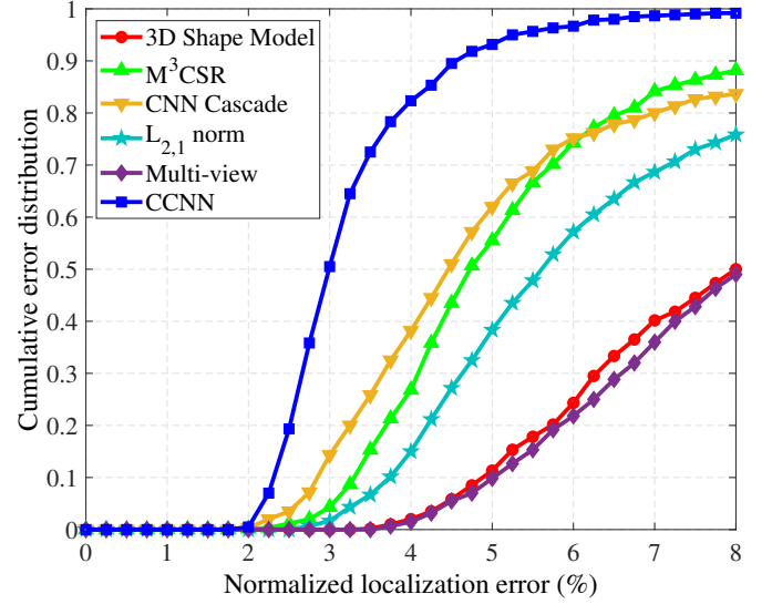
Fig. 9. CEDs vs. NLE results for the 300-W private test set.
