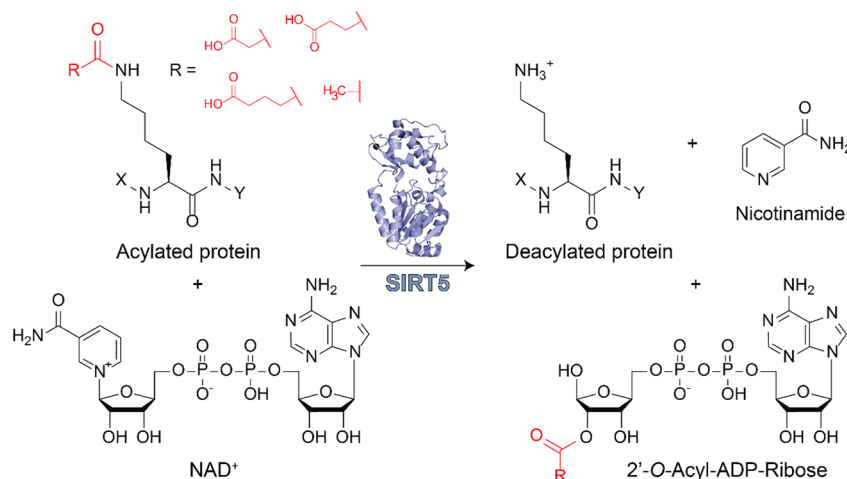
Figure 1. Deacylation reaction catalyzed by SIRT5. The acyl moiety is transferred to the NAD + cosubstrate, yielding the corresponding 2'-O-acyl-ADP-ribose and nicotinamide.
