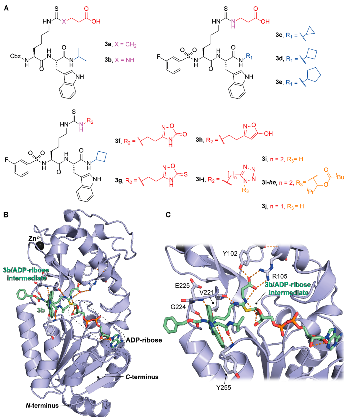
Figure 7. (A) Structures of \epsilon -N-thioglutaryllysine derivatives 3a–j. (B) Structure of hSIRT5 in complex with the ADP-ribose-1'-thioimide intermediate of compound 3b (green) (PDB ID 6EQS). (C) Focus on the binding site to show how the most important residues mediate the protein–compound interaction. Dashed orange lines indicate polar interactions.
