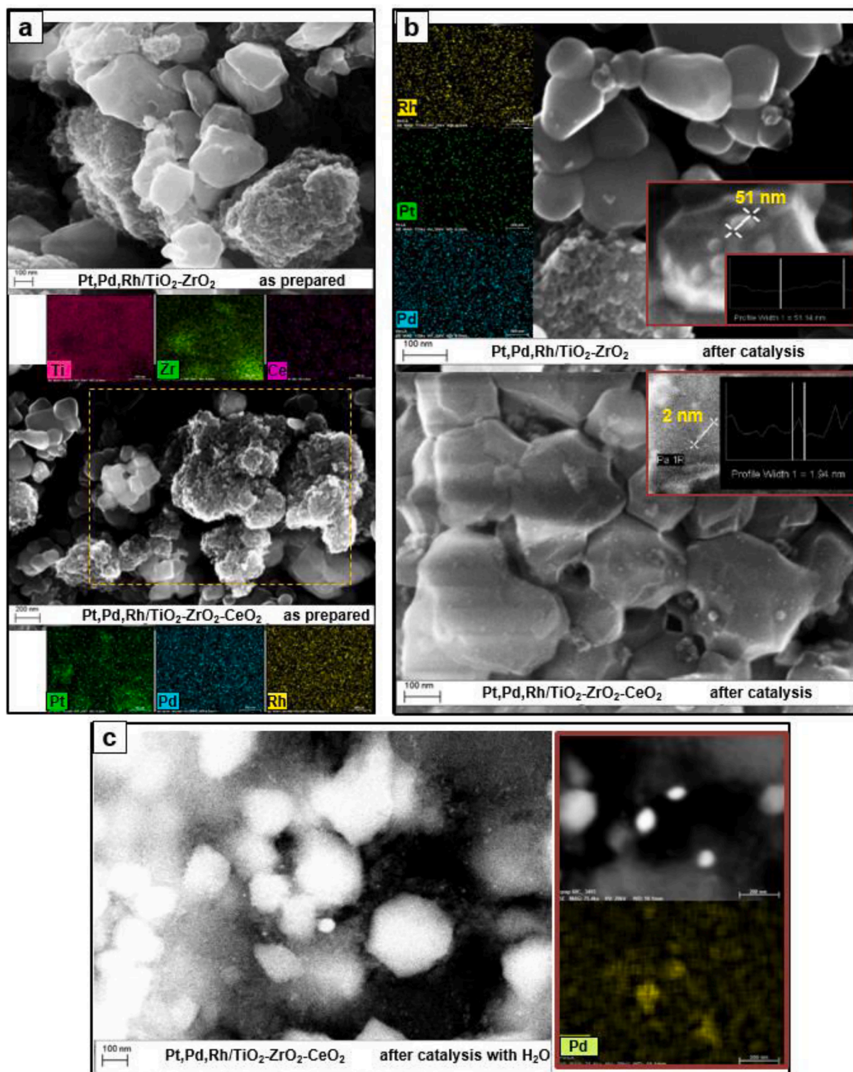
Fig. 2. FESEM images of Pt,Pd,Rh/TiO 2 -ZrO 2 and Pt,Pd,Rh/TiO 2 -ZrO 2 -CeO 2 catalysts as prepared (section a, In-Lens detector) and after the catalytic tests (section b, In-Lens detector) and after catalysis in the presence of H 2 O (section c, Back Scattering detector). The EDX elemental maps (coloured images) are reported in section a (referring to the dotted marked area) for Zr, Ti, Ce, Pt, Pd and Rh, in section b for Pt, Pd and Rh, and in section c for Pd.
