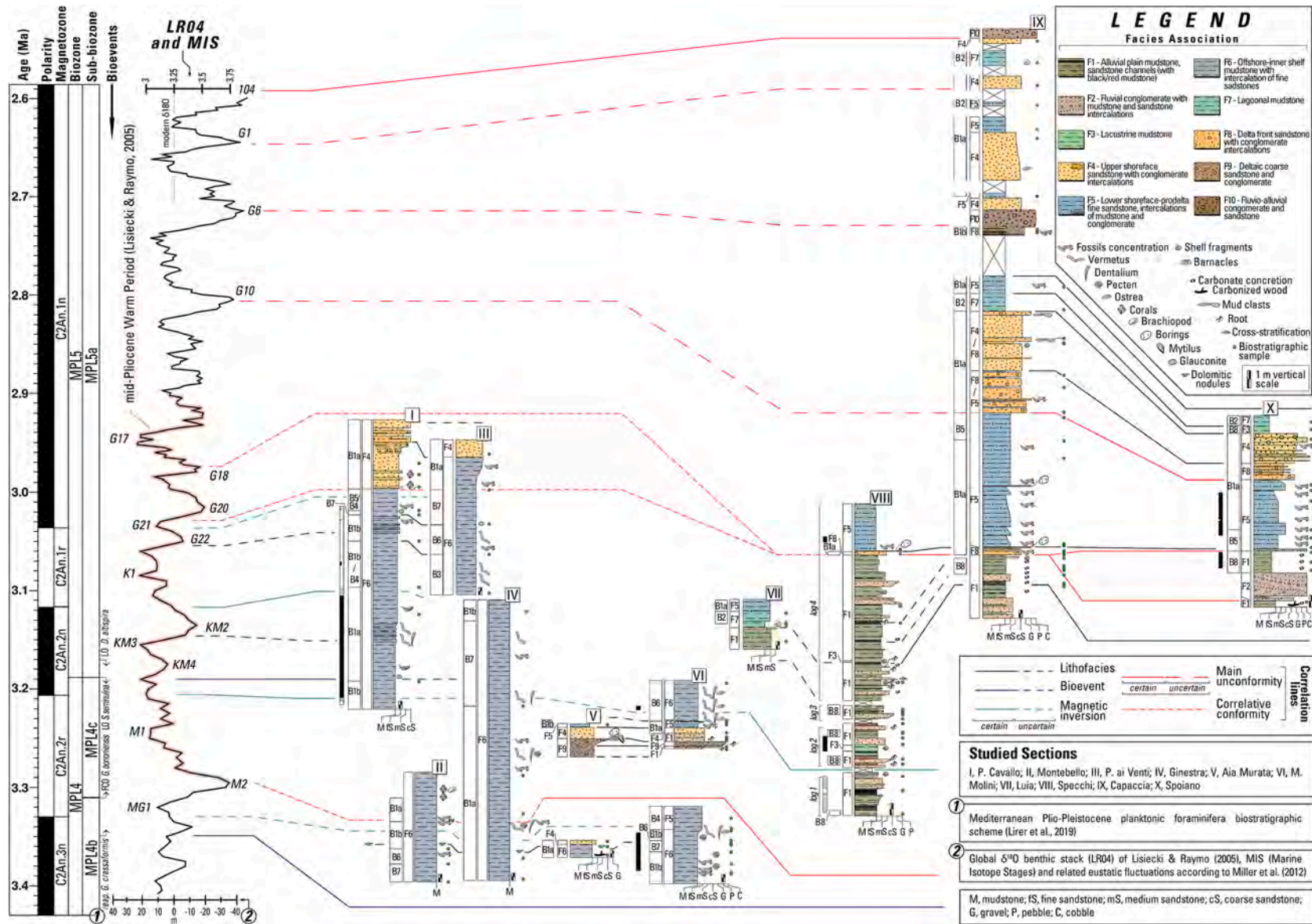
Fig. 5. a, Correlation framework of the studied sections. Biostratigraphy from Lirer et al. (2019). The global benthic \delta^{18}\text{O} stack of Lisiecki and Raymo (2005), scaled to the global eustatic sea level according to Miller et al. (2012). See Table 2 for facies association (F*) and Table 3 for biofacies (B*).
