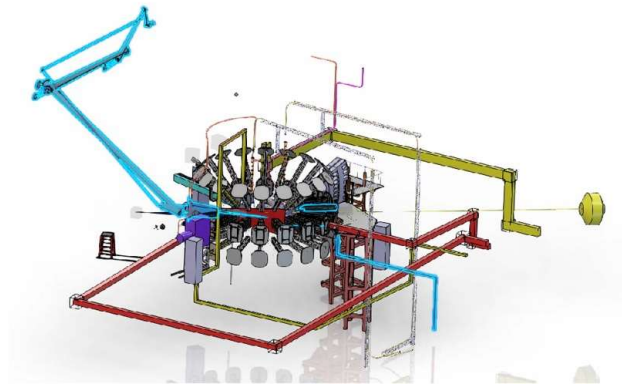
Figure 15. Layout of plasma diagnostics in 3D CAD model showing that each diagnostic system is already fully integrated in the design. Reproduced with permission from DTT team.
