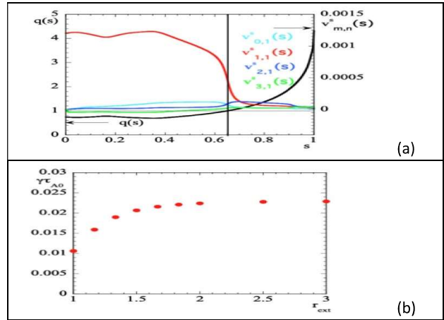
Figure 2. Stability characteristics. (a) Dominant contravariant Fourier components of the perturbed velocity v_{m,n}^s for the internal kink mode safety factor q versus s (where s \sim (\text{psi})^{1/2} is the normalized radial-like coordinate, and \text{psi} the poloidal flux function) at r_{\text{ext}} = 3 . (b) Internal kink growth rate, normalized to the inverse of the on axis Alfvén time \tau_{A0} ( \tau_{A0} = R_0(\mu_0 \rho_0)^{1/2}/B_0 ), \rho_0 is the on axis mass density) versus the normalized distance r_{\text{ext}} of the perfectly conducting wall. Reproduced with permission from [17].
