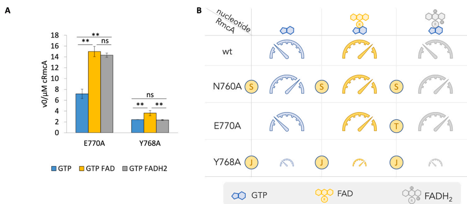
Fig. 6. FAD-dependence of PDE kinetics in different cRmcA mutants. (A) Initial velocity v_0/\mu\text{M} enzyme obtained at 30 \mu\text{M} c-di-GMP with cRmcA variants indicated in the X-axis, in the presence of 100 \mu\text{M} GTP (blue bars), 50 \mu\text{M} FAD (yellow bars) and FADH 2 (grey bars). Data are the mean of at least four experiments \pm SD. In E770A, grey bar is not significantly different from the corresponding yellow one (P value > 0.01); in Y768A, grey bar is significantly different from the corresponding yellow one (P value < 0.001). (B) A cartoon summarizing the kinetics profile of wt cRmcA and the different mutants relevant to the redox-dependent tuning of PDE activity. The effect on the PDE activity tuning is depicted as a tachometer: Low PDE or High PDE are depicted with the needle on the left or on the right, respectively. Small tachometer cartoons for Y768A mutant refers to an overall reduced turnover as compared to the wt. The label with circled letters indicates the role identified for each key residue in FAD/FADH 2 redox-switch, according to the corresponding mutant kinetics behavior. In particular, (S) for sensing redox state, (T) for signal transduction, (J) for Joint.
