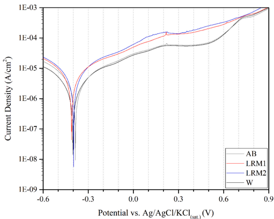
Fig. 22. Polarization curves of samples with different substrate surface conditions subjected to electrochemical polarization testing in 3.5 w/v% NaCl aqueous solution.
