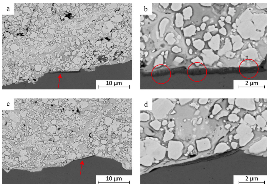
Fig. 12. SEM micrographs (backscattered electrons) showing details of the coating-substrate interface in the AB (a, b) and LRM1 sample (c, d). Red arrows = interface oxide. Red circles = cracks.
