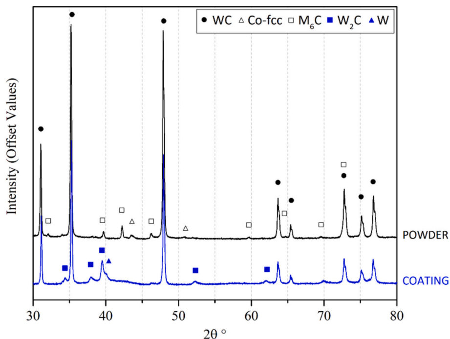
Fig. 11. XRD patterns of the feedstock powder (black line) and the coating (blue line). Reference patterns: WC (JCPDF 51-939), Co-fcc (JCPDF 15-806), M6C (JCPDF 27-1125), W2C (JCPDF 37-776), W (JCPDF 4-806).
