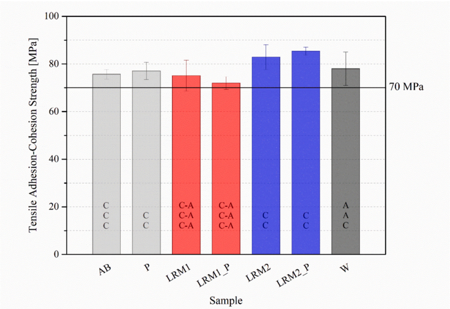
Fig. 18. Results of tensile adhesion tests on the coatings sprayed onto the L-PBF samples. Failure modes in each test are listed on the bars: “A” = adhesive failure, “C” = cohesive failure.
