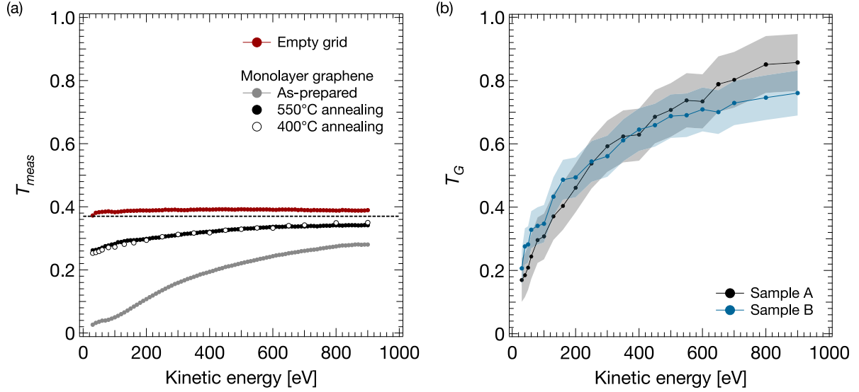
Fig. 6. (a) Measured transmission of electrons through an empty TEM grid (red) and through as-prepared (grey), 550 °C annealed (black markers) and 400 °C annealed (open markers) monolayer graphene on TEM grid. The dashed line is the 37% geometrical transmission of the TEM grid supporting the graphene, evaluated with SEM images analysis. (b) Corrected graphene transmission through the 400 °C annealed monolayer graphene (black) and a second annealed monolayer graphene (blue). The shaded areas represent the uncertainty associated with the respective T_G measurements. (For interpretation of the references to colour in this figure legend, the reader is referred to the web version of this article.)
