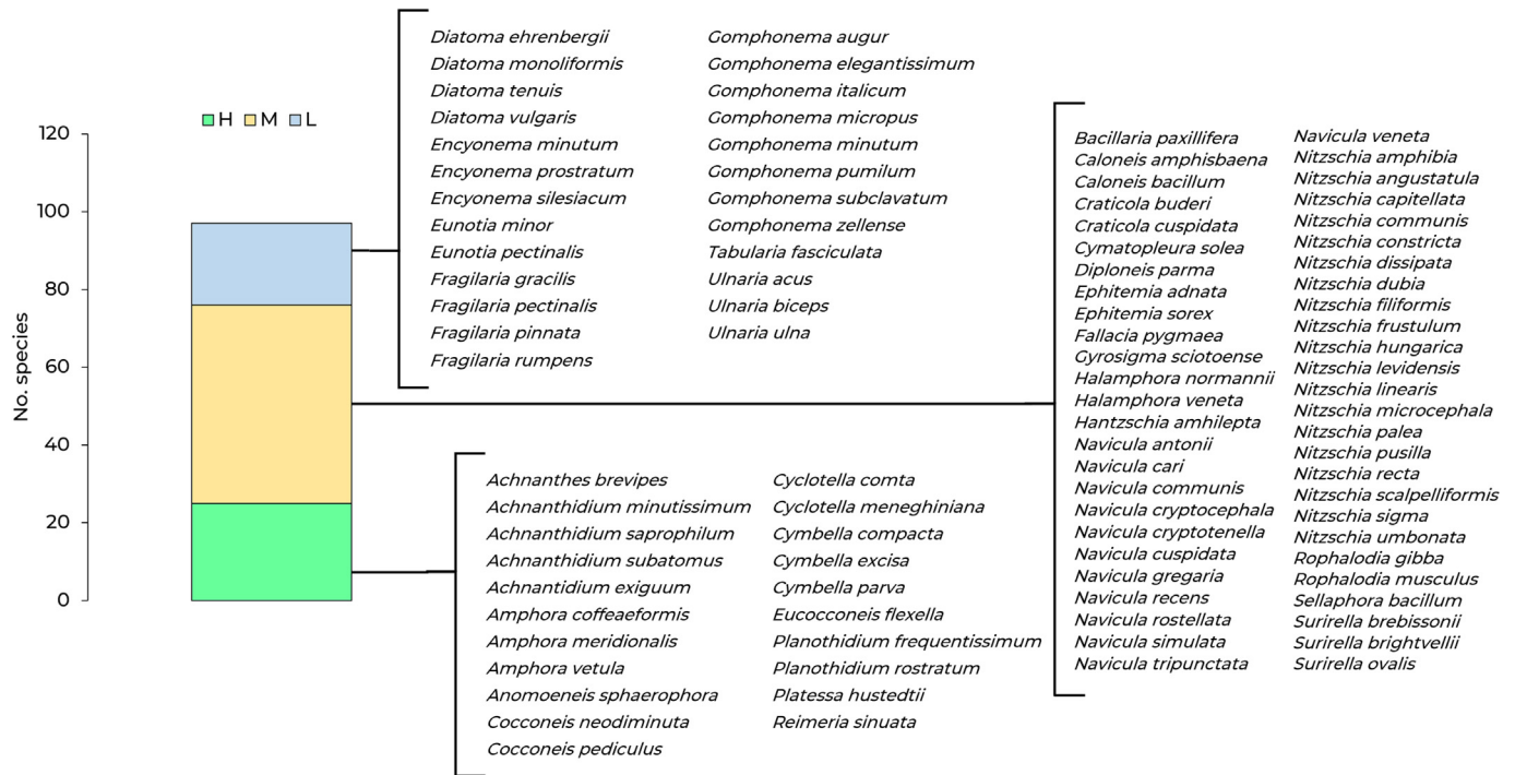
Fig. 3. Number of species (No. species) belonging to “High profile” guild (H), “Low profile” guild (L) and “Motile” guild (M) and relative species found.
