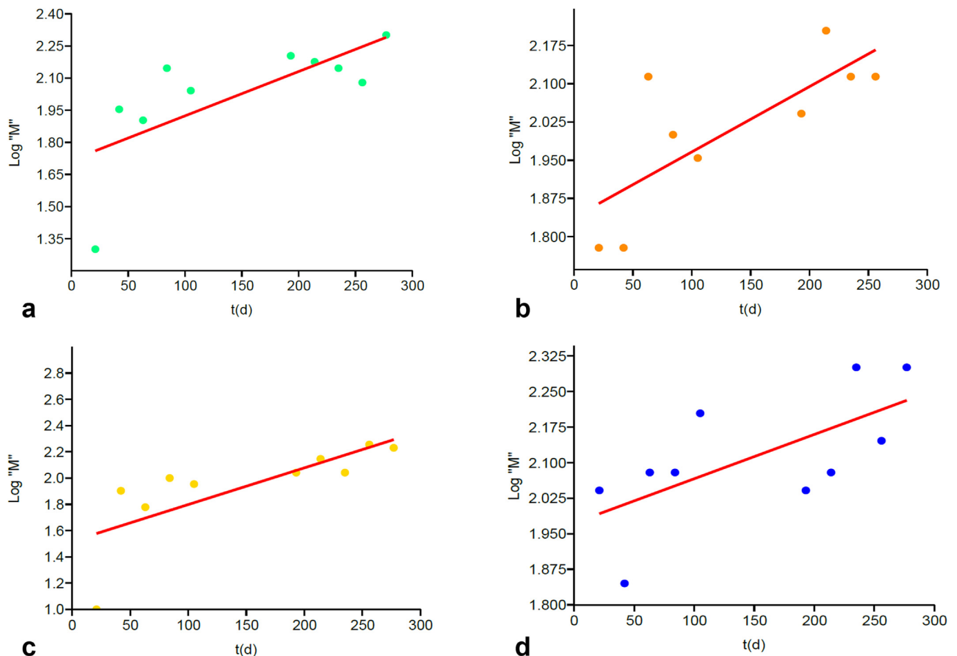
Fig. 4. Plot of log transformed data showing the regression line as regards the number of species belonging to the “Motile guild” calculated for fPS (a), dPS (b), fPE (c) and dPE (d). Log “M”: Logarithm of “Motile” guild values; Time is expressed in days (PAST).
