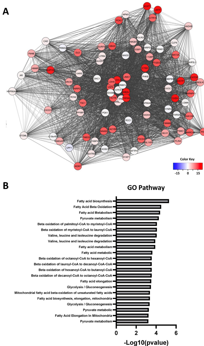
Figure 2: Interactome of AR. A) AR interaction network of the C4-2 CRPC cell line. Proteins identified by AR pulldown assay after treatment with MC3324 (25 \mu\text{M} ) were annotated and clustered. B) GO term annotation for metabolic functions associated with AR interactors.
