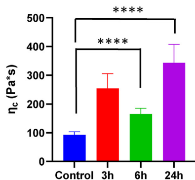
Figure 7: Mechanical and physical properties. MC3324 alters the viscoelastic properties of PC3 cells. A) PC3 culture inside the AFS chip at different time points of MC3324 exposure. B) Example traces of PC3 creep compliance at different time points of MC3324 exposure. C) Graph showing that MC3324 significantly increases the average elastic modulus E_a in a time-dependent manner ( p < 0.0001 ). D) Graph showing that MC3324 significantly increases the average viscosity \eta_a in a time-dependent manner ( p < 0.0001 ). E) Graph showing that the average background viscosity \eta_c of PC3 cells significantly increases upon stimulation by MC3324 in a time-dependent manner ( p < 0.0001 ).
