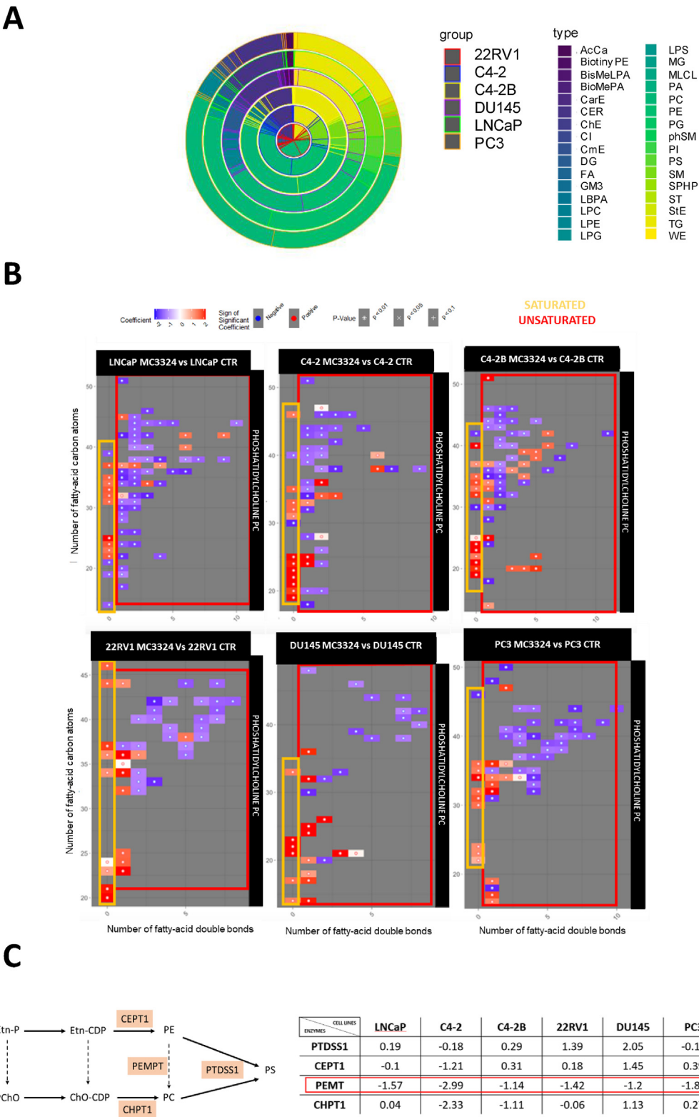
Figure 6: Lipid content alteration. A) Multiple pie chart showing relative lipid class content in prostate cell lines. The six rings correspond to different PCA cell lines: 22RV1 (red), C4-2 (blue), C4-2 B (yellow), DU145 (violet), LNCaP (green), PC3 (orange); for each cell line, relative lipid class subgroups are highlighted with different colors inside the circle. B) Phosphatidylcholine (PC) species based on saturation degree (x axis) and length of fatty acid (y axis) grouped by saturated (yellow) and unsaturated (red) matrix. C) Enzymes involved in phosphatidylserine (PS) synthesis from phosphatidylethanolamines (PE) or phosphatidylcholines (PC). Relative expression of PTDSS1 , CEPT1 , PEMT , and CHPT1 genes from real-time PCR data after MC3324 treatment for 24 h in the indicated PCA cell lines. Experiments were performed in triplicates.
