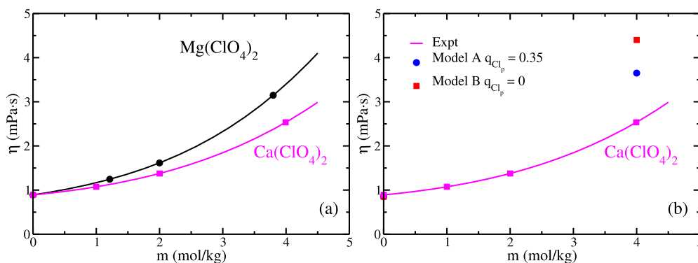
Fig. 3. (a) Experimental shear viscosity curves as a function of concentration for aqueous \text{Mg}(\text{ClO}_4)_2 (black solid line) and \text{Ca}(\text{ClO}_4)_2 (magenta line) solutions at 298.15 K and 1 bar. (b) Simulation results for viscosities using Model A with q_{\text{Cl}_p} = 0.35e (blue circles) and model B with q_{\text{Cl}_p} = 0e (red squares).
