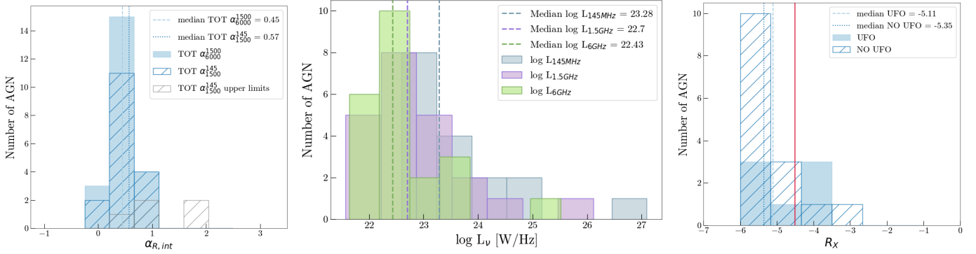
Fig. 4. Left: Spectral index distribution of the sample. The filled histogram represents the values computed between 1.5 and 6 GHz, while the barred one those computed between 145 MHz and 1.5 GHz. Middle: Histogram comparing the total radio luminosities of the sample. Blue: 145 MHz. Violet: 1.5 GHz. Green: 6 GHz. The upper limits at 145 MHz have been excluded. Right: Radio loudness parameter distribution of the sample. The convention followed is R_X = \log(L_R(6\text{ cm})/L_X(2-10\text{ KeV})) (Terashima & Wilson 2003). The filled histogram represents the values of R_X computed for the UFO hosts, and the barred histogram those derived for the non-UFO hosts. The vertical red line marks the -4.5 limit set by Terashima & Wilson (2003). RQ AGNs tend to dominate the sample, while RL AGNs represent only a small fraction, specifically 6/21 with the original limit R_X = -4.5 .
