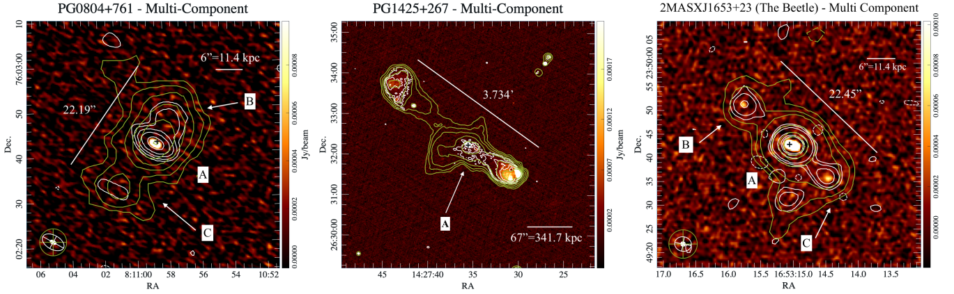
Fig. 2. Images of the ‘multi-component’ sources. Colours at 6 GHz with \sigma_{rms} \cdot [-3, 3, 6, 12, 24, 48, 96] contours at 1.5 GHz (white) and 145 MHz (green). The beams are shown in the bottom-left corner of each panel. Labels A, B, and C mark distinct radio components: A denotes the nuclear (core) component spatially coincident with the optical AGN position, while B and C denote spatially-separated extranuclear components (i.e. features that are not coincident with the optical/IR nucleus and that extend beyond the host’s optical light profile) likely related to AGN outflows.
