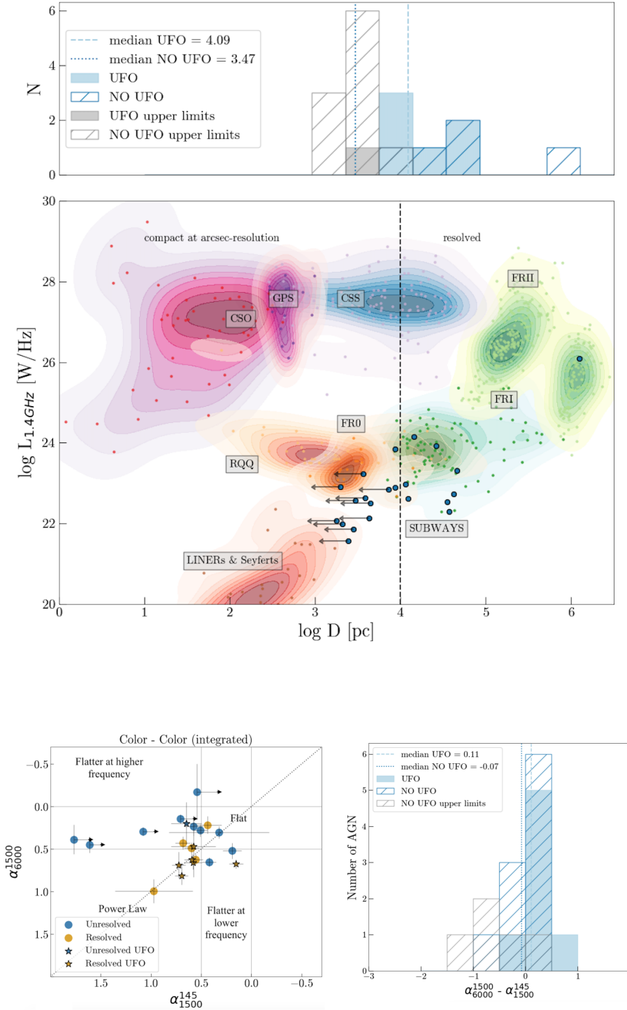
Fig. 5. Radio power at 1.4 GHz versus linear size plot (P-D diagram) for different types of RL and RQ AGNs, adapted from Baldi (2023). Points show individual objects and coloured contours represent a smoothed estimator of source density. The different categories of source shown are: CSO (compact symmetric objects), GPS (GHz-peaked spectrum sources), CSS (compact steep spectrum sources), FRI, FRII, RQ quasars, Seyferts and LINERS, and FR0s. The vertical dashed line roughly marks the separation between resolved and unresolved compact sources based on arcsecond angular resolution. The blue dots represent how SUBWAYS AGNs overlap to LINERS & Seyferts, FRI, FR0s and RQQ. PG1425+267 is a strong outlier, falling on the FRII region. Such variety is consistent with the sample being selected based on its X-ray properties. In the upper panel we show the linear size distribution of the sample, with the UFO subsample (filled histogram) separated from the non-UFO one (barred histogram). The median physical size measured for the UFO subsample is higher ( 12.35 \pm 5 kpc) with respect to the non-UFO one ( 2.96 \pm 1 kpc), potentially supporting multi-phase outflow models (e.g. Crenshaw et al. 2003). Medians are computed taking into account the upper limits through KM survival analysis. Catalogue references: LINERS & Seyferts (Baldi et al. 2018), FR0 (Baldi et al. 2019; Cheng & An 2018); RQQ (Jarvis et al. 2021); GPS (Liu et al. 2007); CSS (Kunert-Bajraszewska et al. 2010); CSO (An & Baan 2012); FRI (Dabhade et al. 2020; Jimenez-Gallardo et al. 2019); FRII (Lao et al. 2024; Fanti et al. 1987).
