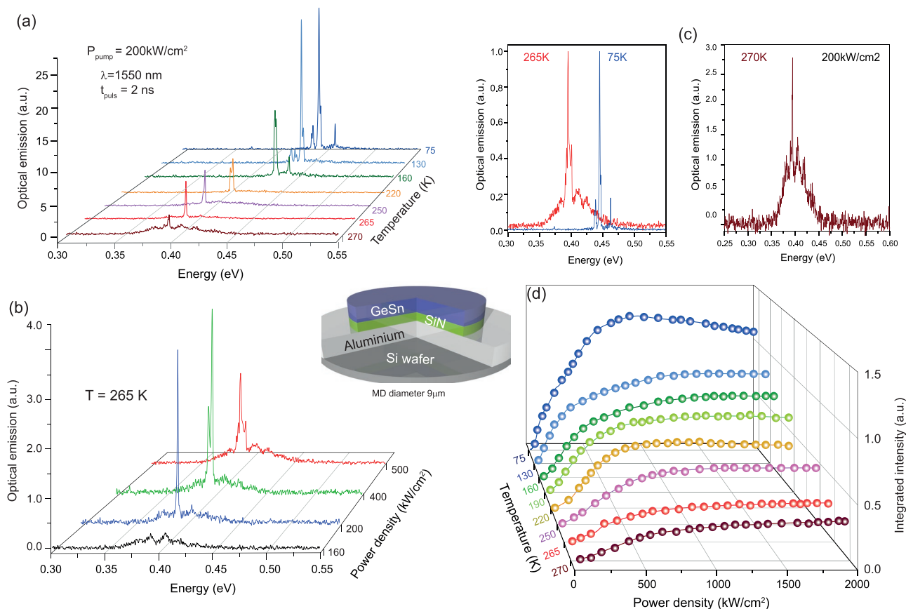
Figure 3. Strain relaxed microdisks. Laser properties of relaxed 9 μm diameter GeSn mesa micro-disks MMD. a) Temperature dependence of the PL emission under 200 kW cm -2 optical pumping. b) Power dependence of the PL spectra at 265 K. c) Laser spectra for 200 kW cm -2 optical pumping at 75, 265, and 270 K. d) Temperature dependent L–L characteristic. Very weak roll-off is seen with increasing pumping power.
