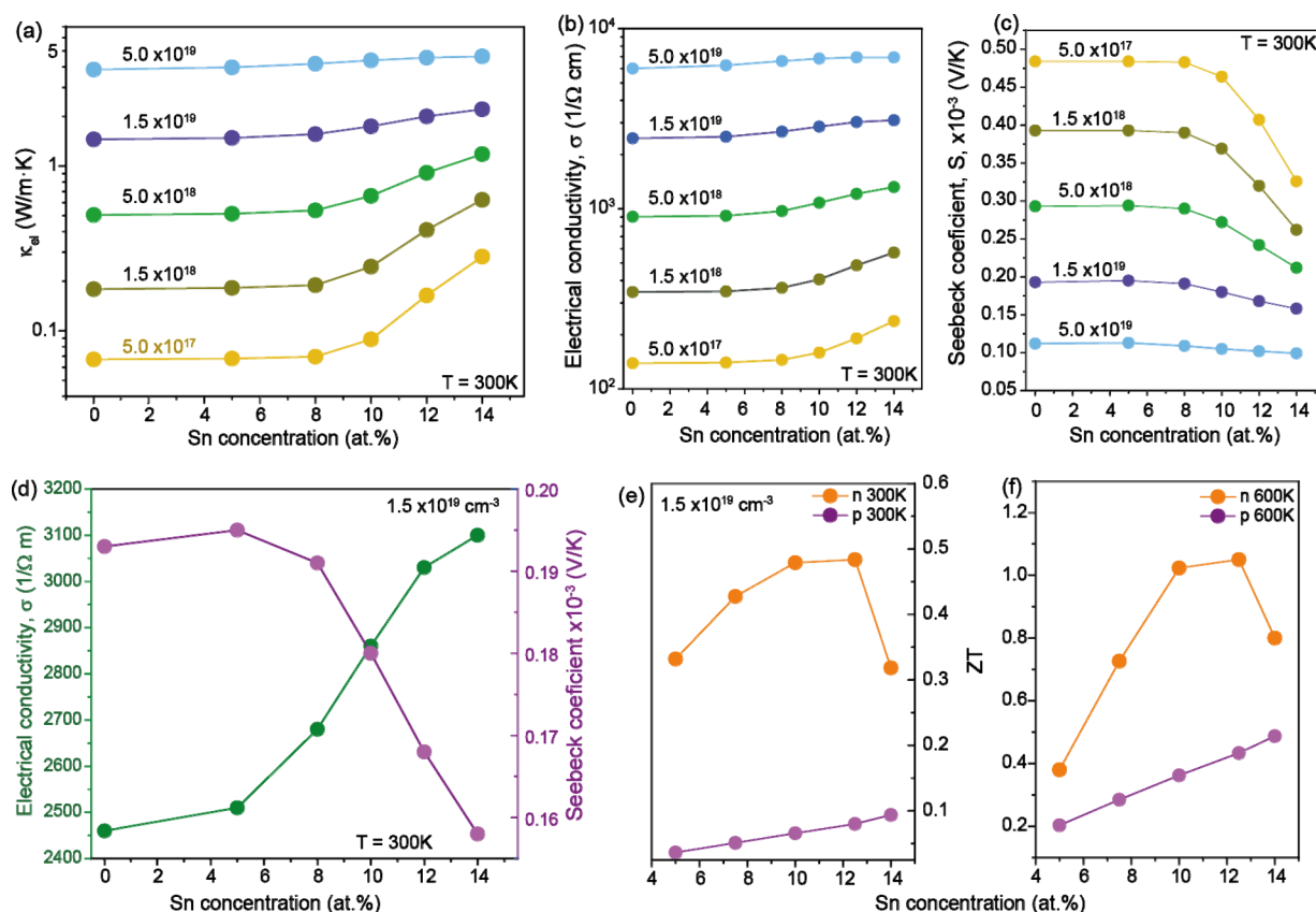
Figure 4. TE parameter modeling. (a) Electronic thermal conductivity \kappa_e , (b) electrical conductivity \sigma , and (c) the Seebeck coefficient S , as a function of Sn content for different n-type doping concentrations at 300 K. (d) The charge transport coefficients for different Sn contents for n-type doping of 1.5 \times 10^{19} \text{ cm}^{-3} , indicating the opposite behavior of \sigma and S . (e, f) ZT at a carrier density of 1.5 \times 10^{19} \text{ cm}^{-3} versus Sn composition, for p-type and n-type GeSn alloys at temperatures of (e) 300 K and (f) 600 K.
