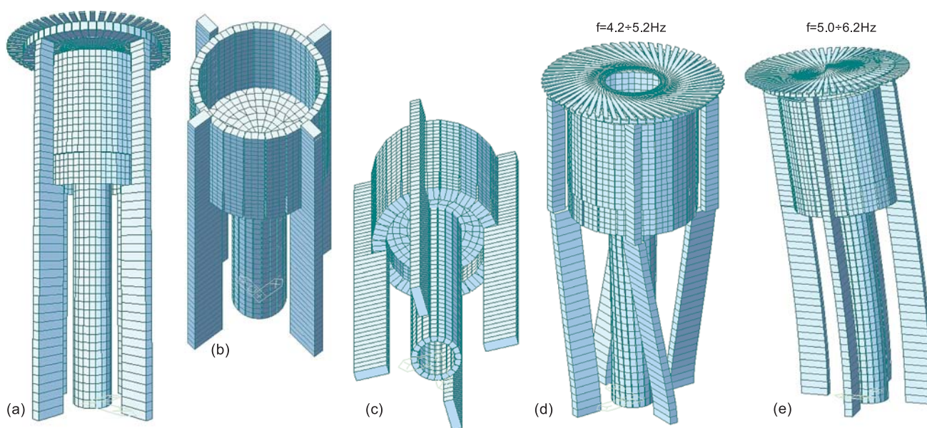
Fig. 6 Overview of the numerical model (a), detail of the elevated tank (b) and of the cylindrical central columns (c), and modal shapes for the torsional (d) and flexural (e) vibration modes
