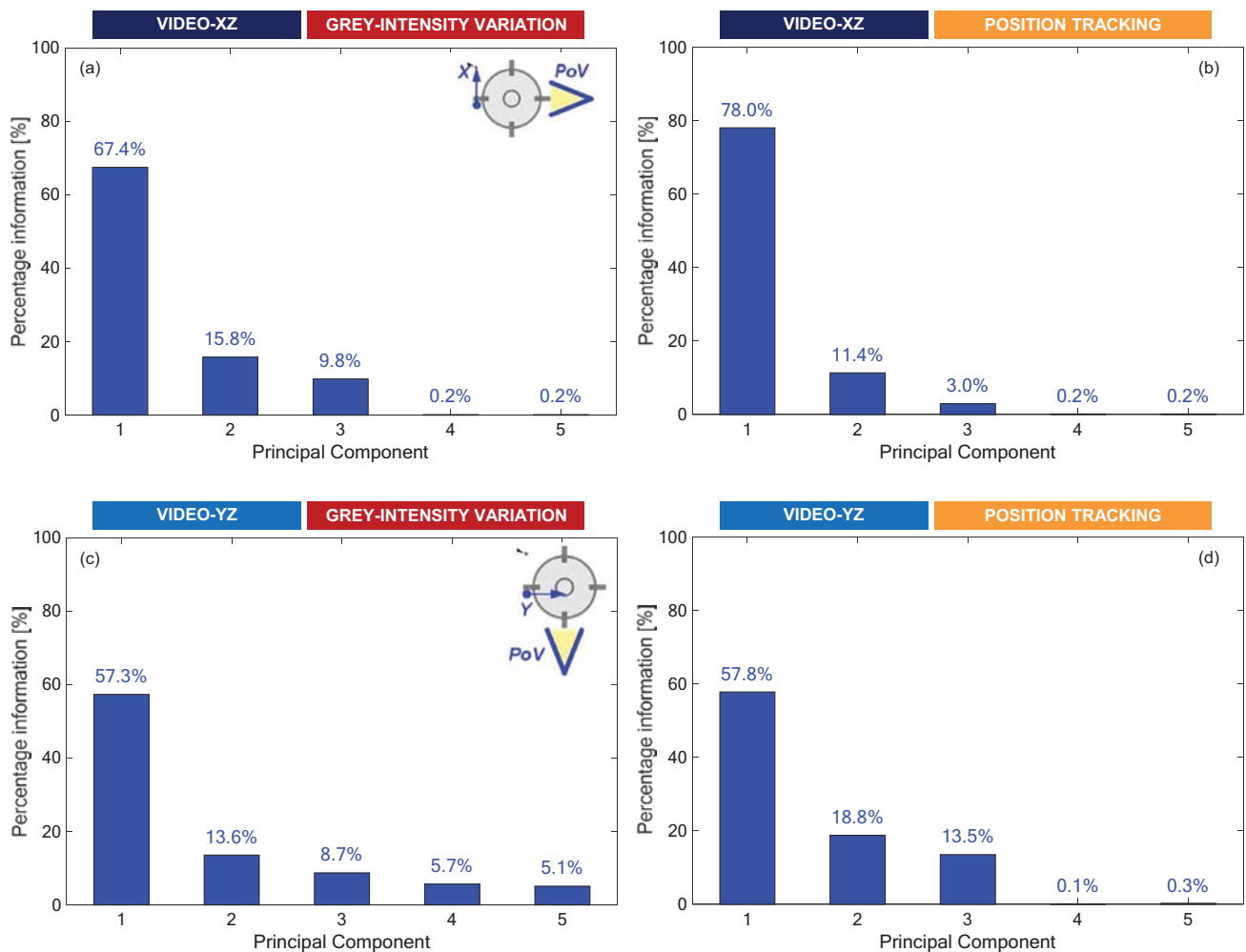
Fig. 11 Content of the first five principal components from pixel grey-intensity variation (a, c) and from pixel position tracking (b, d) analyses for Video-XZ (a, b) and for Video-YZ (c, d)
