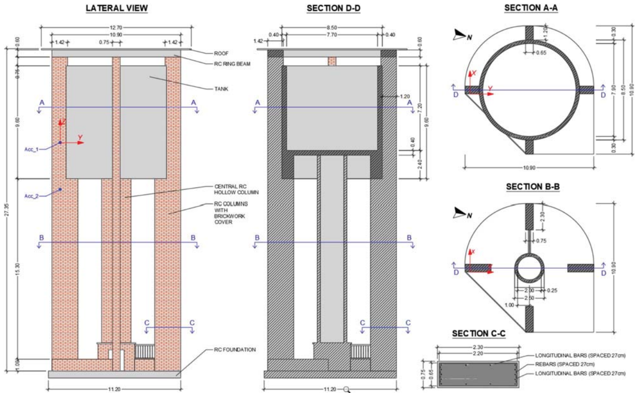
Fig. 2 Lateral view, and vertical and horizontal cross sections of Tiburtina elevated water tank
