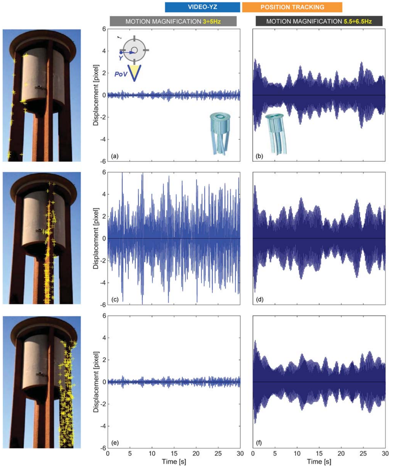
Fig. 15 Time histories of horizontal displacements derived from pixel position tracking analyses on Video-YZ, amplified in the frequency range 3 \div 5 Hz, for pixels selected in the left (a, b), central (c, d) and
