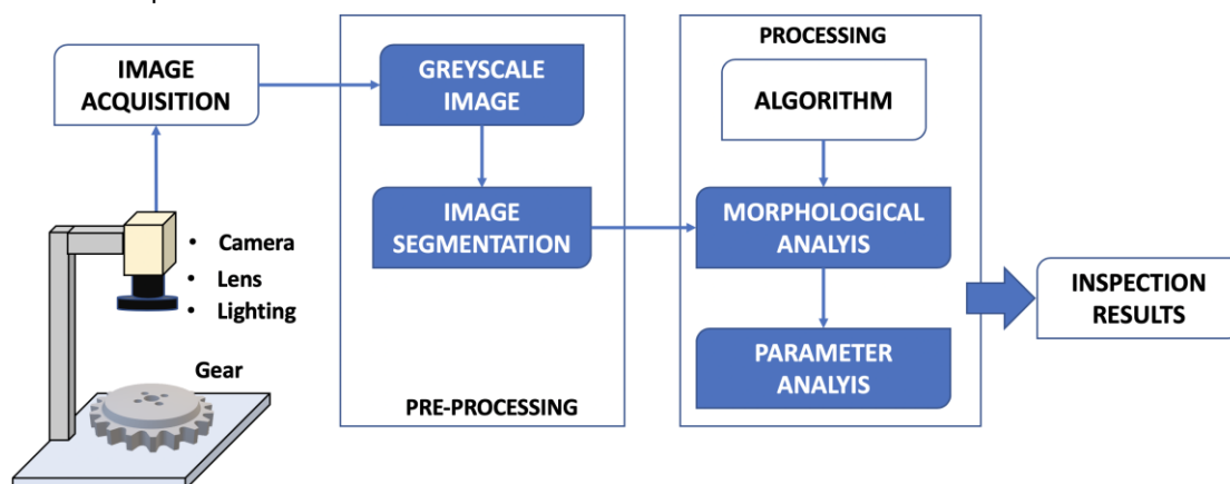
Figure 3: Camera-inspection process.
