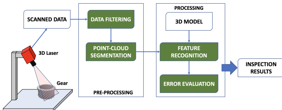
Figure 4: 3D Laser scanning process.
