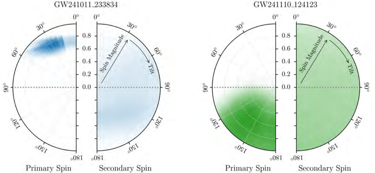
Figure 12. Posterior on both the primary and secondary spin vectors of GW241011 (left) and GW241110 (right). As in Figure 2, radial and polar coordinates correspond to dimensionless spin magnitude vectors and spin-orbit misalignment angles, respectively. Pixels spaced uniformly in spin magnitude and in cosine-tilt angles, such that each pixel contains equal prior probability. For both events, the properties of the secondary spin vectors are unconstrained.
