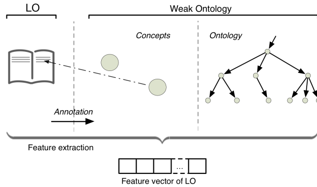
Figure 3: Each LO is being assigned to a feature vector.
