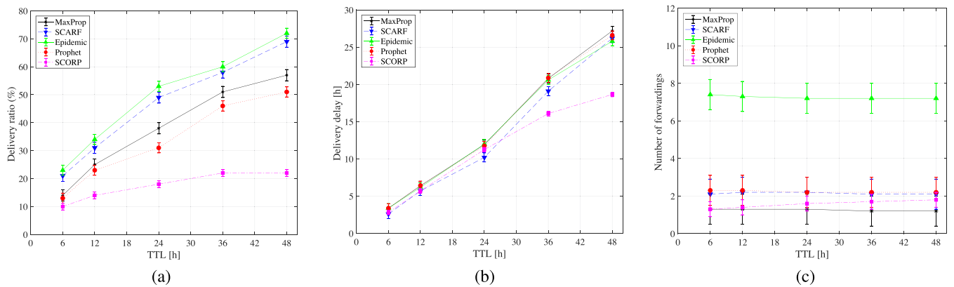
Fig. 14. Synthetic trace scenario with 20 vehicles. Simulation results for (a) delivery ratio, (b) delivery delay, and (c) average cost, versus TTL.
