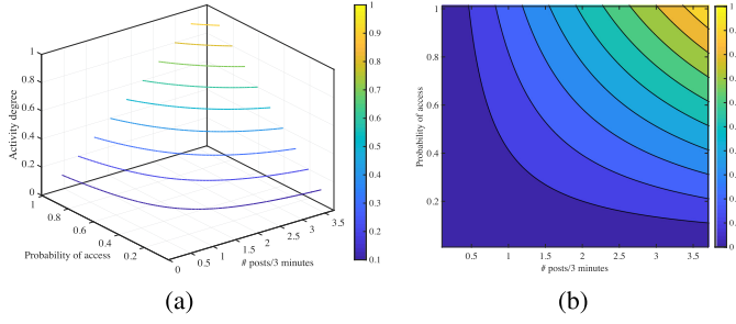
Fig. 4. (a) Contour plot of activity degree versus the number of posts over 3 minutes i.e., [0, 3.6] , and the probability of accessing the vehicular social network i.e., [0, 1] . (b) Top-view of the activity degree.
