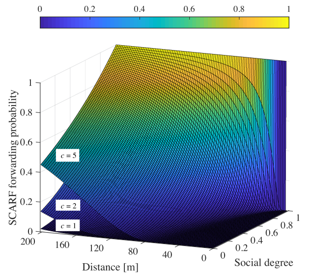
Fig. 9. SCARF forwarding probability versus the distance d [m] (with d \leq z ) and the social degree. In this case, we assumed \rho = 0.02 [veh/m] and different values of the shape factor, i.e., c_i = [1, 2, 5] .
