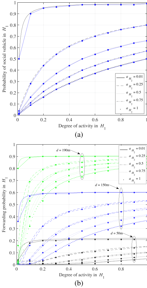
Fig. 12. (a) Analytical (black lines) and simulated (blue lines) results of the probability of social vehicle. (b) Analytical (no marker lines) and simulated (lines with star marker) results of the probability of forwarding of a vehicle versus the degree of activity under the hypothesis H_1 , for different distances and a_{H_2} values.
