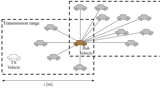
Fig. 2. Schematic of a VSN comprised of two clusters (dotted areas). The hub vehicle (brown vehicle) has a higher network degree and will be likely to disseminate an information packet to a large number of neighboring vehicles. From a social networking perspective, a hub vehicle is a social node with high activity degree.
