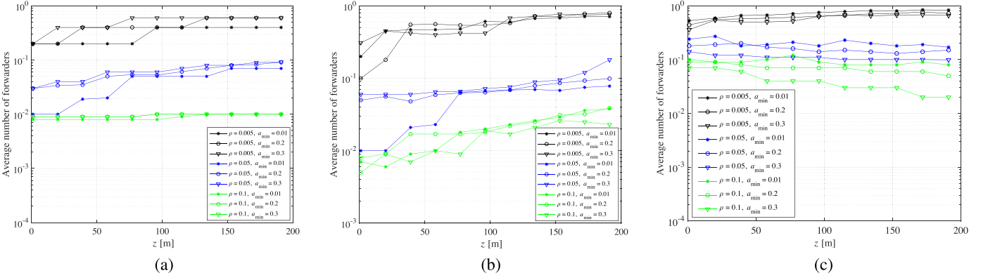
Fig. 17. Simulation results of the average number of forwarders within a source node transmission range, for (a) 20-vehicle synthetic trace ( Helsinki scenario ), (b) 40-vehicle synthetic trace ( Helsinki scenario ), and (c) 370-taxi real trace scenario ( Rome taxi scenario ).
