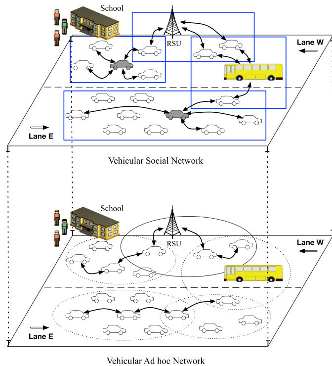
Fig. 1. Mapping between VANET and VSN. In VANET, next-hop vehicles are selected within a transmission range (dotted circles) according to a greedy algorithm. In VSNs, vehicles are distinguished according to social features (i.e., social degree). Vehicles are members of a VSN (blue rectangles), if they share common interests. Social nodes (grey vehicles) are preferably selected as next-hop forwarders in order to reach more nodes.
