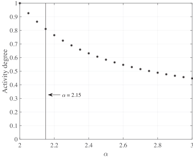
Fig. 5. Activity degree versus \alpha . The threshold A = 0.8 is set for \alpha = 2.15 .
