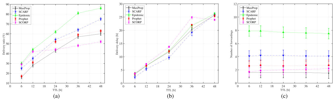
Fig. 15. Synthetic trace scenario with 40 vehicles. Simulation results for (a) delivery ratio, (b) delivery delay, and (c) average cost.
