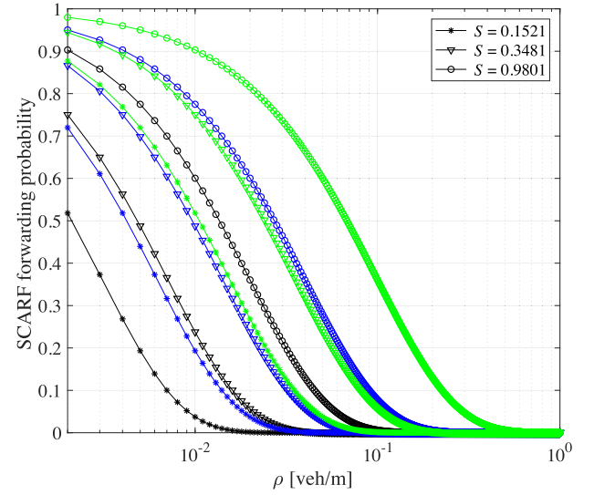
Fig. 8. SCARF forwarding probability for a vehicle within the source vehicle's transmission range z [m], versus the vehicular density \rho [veh/m] and for selected values of the social degree and of the shape factor, i.e., c = [1, 2, 5] for black, blue and green lines, respectively.
