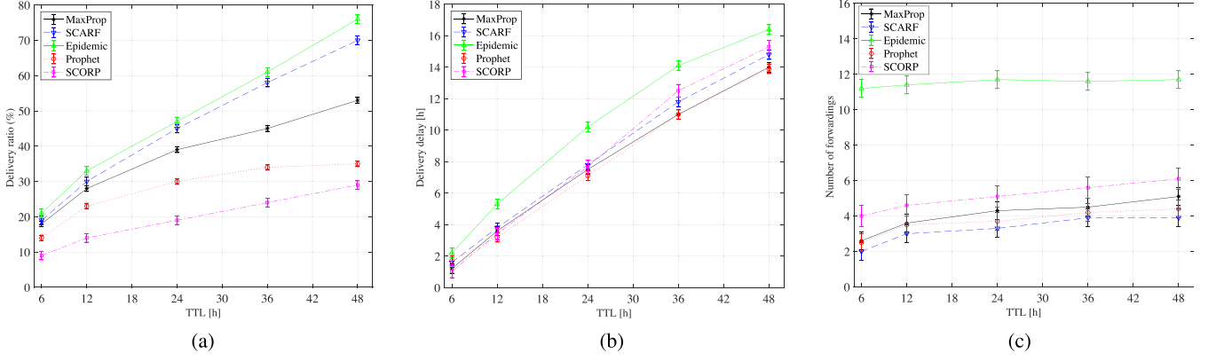
Fig. 16. Real trace scenario with 370 taxis from Roma city [45]. Simulation results for (a) delivery ratio, (b) delivery delay, and (c) average cost.
