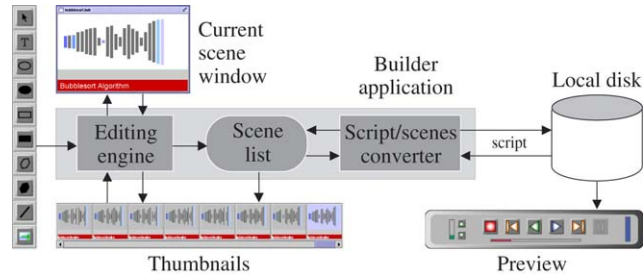
Fig. 5. Internal organization of the Builder.
