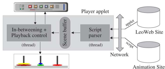
Fig. 4. Internal organization of the Player.
