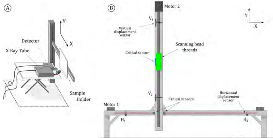
Figure 2. Translation stages: portable version (A) and mobile version (B).
