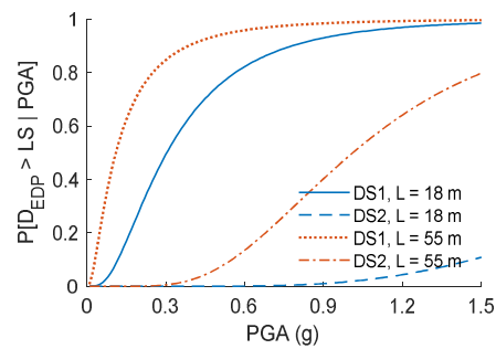
Figure 8. Fragility curves for DS1 and DS2 of the column with the lower and upper values of the span length.
