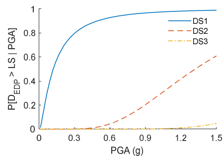
Figure 6. Fragility curves for different damage states of the column considering the range of the input random variables in Table 1.
