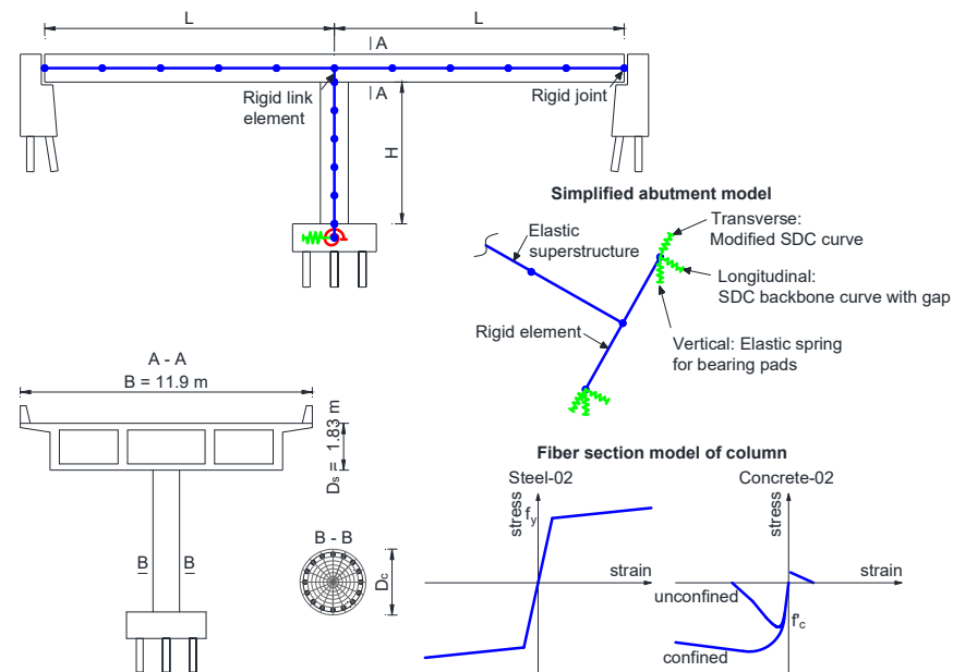
Figure 2. Two-span, single-bent RC bridge model.
