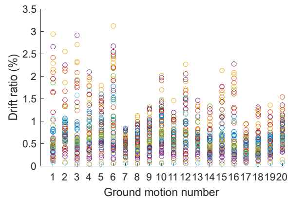
Figure 5. Maximum column drifts collected as observed training data.
