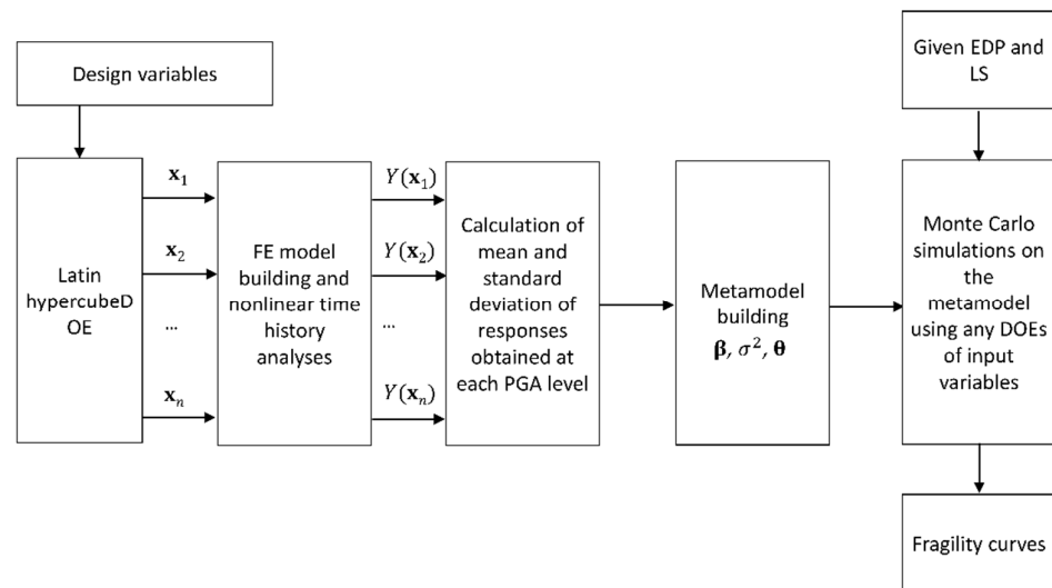
Figure 1. Kriging metamodel-based fragility evaluation procedure.
