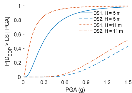
Figure 7. Fragility curves for DS1 and DS2 of the column with the lower and upper values of the column height.
