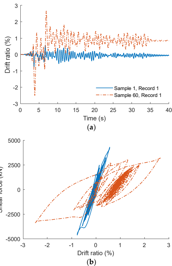
Figure 4. Example of nonlinear time history analysis results: (a) Time history data of column top drift ratio and (b) Hysteretic behavior in terms of column top drift ratio and base shear.
