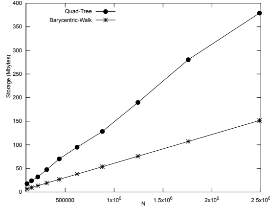
Figure 8: Memory storage (Mbytes) required for quadtree (black circles) and barycentric walk (crosses), for 10^5 \lesssim N \lesssim 2.5 \cdot 10^6 .
