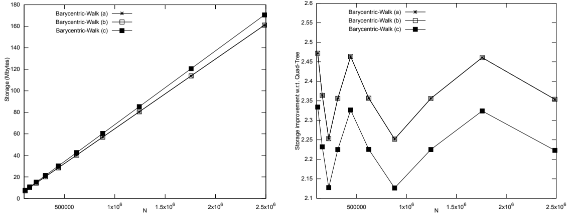
Figure 9: Memory storage (Mbytes) required by the initialization strategies for the barycentric walk (left) and improvement w.r.t. storage for the quadtree, for 10^5 \lesssim N \lesssim 2.5 \cdot 10^6 . Strategy (BWa): crosses, strategy (BWb): white squares, strategy (BWc): black squares.
