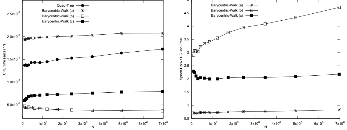
Figure 11: Averaged search time of the quadtree and barycentric walk (left) and improvement factor versus the quadtree search (right), for 10^5 \lesssim N \lesssim 7 \cdot 10^6 . Strategy (BWa): crosses, strategy (BWb): white squares, strategy (BWc): black squares, quadtree: black circles.
