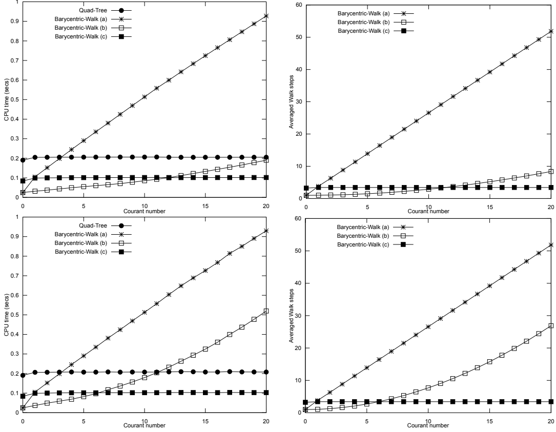
Figure 12: Search times versus Courant number (left) and averaged barycentric walk steps versus Courant number (right), for N = 1.5 \cdot 10^6 , L_x = 2\pi , and with L_t = 2\pi (upper plots), L_t = 8\pi (lower plots). Strategy (BWA): crosses, strategy (BWb): white squares, strategy (BWc): black squares, quadtree: black circles.
