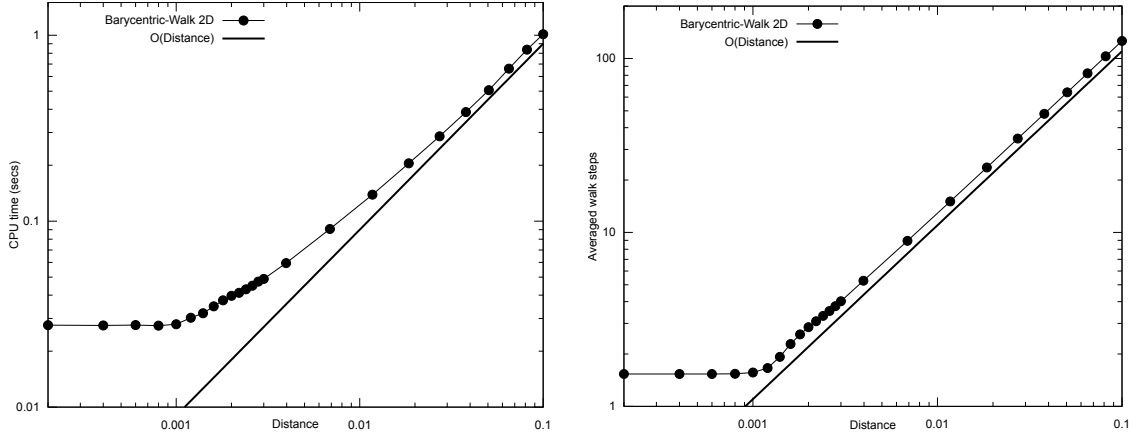
Figure 6: Execution times (left) and averaged walk steps (right) for the barycentric walk search on the whole mesh ( d = 2 , N \sim 4 \cdot 10^5 ), versus distance between start and end points, compared with the line of linear increase.
