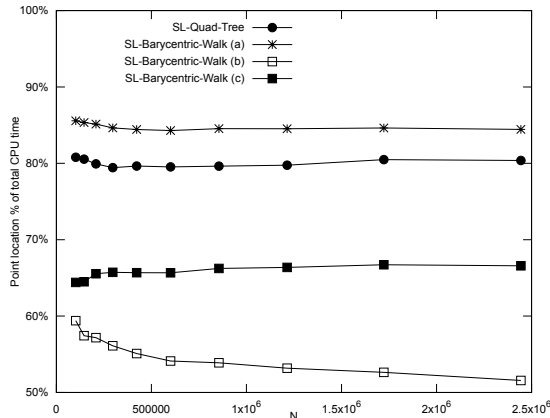
Figure 17: Fraction of CPU time used for point location, for different algorithms in a SL scheme, versus number of grid nodes 10^5 \lesssim N \lesssim 2.5 \cdot 10^6 . Strategy (BWa): crosses, strategy (BWb): white squares, strategy (BWc): black squares, quadtree: black circles.
