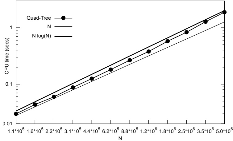
Figure 3: Execution times for the quadtree search on the whole mesh, compared with N and N \log N curves, for 10^5 \leq N \leq 5 \cdot 10^6 .
