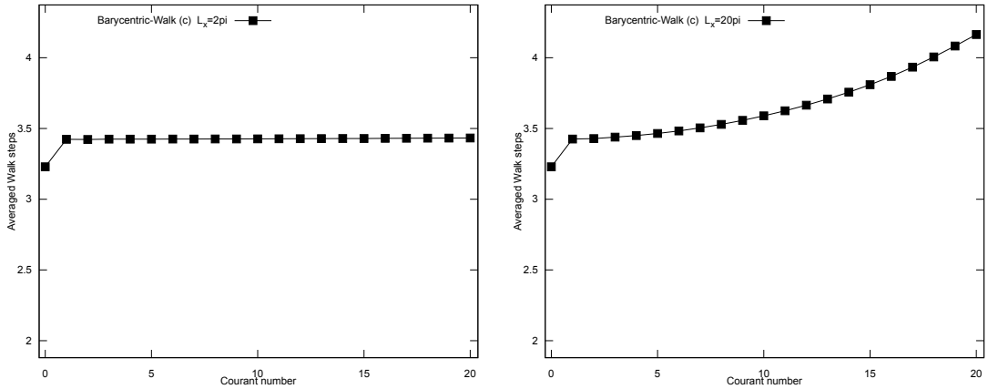
Figure 13: Averaged barycentric walk steps versus Courant number for strategy (BWc), with N = 1.5 \cdot 10^6 and L_x = 2\pi (left), L_x = 20\pi (right).
