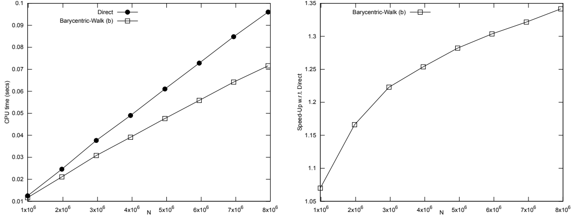
Figure 15: Search time (left) and improvement factor (right) of the barycentric walk with initialization strategy (BWb) versus the direct search on a structured grid, for 10^6 \lesssim N \lesssim 8 \cdot 10^6 . Direct access: black circles, strategy (BWb): white squares.
