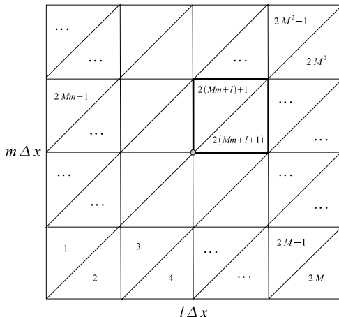
Figure 14: Courant triangular grid for structured/unstructured search comparison.
