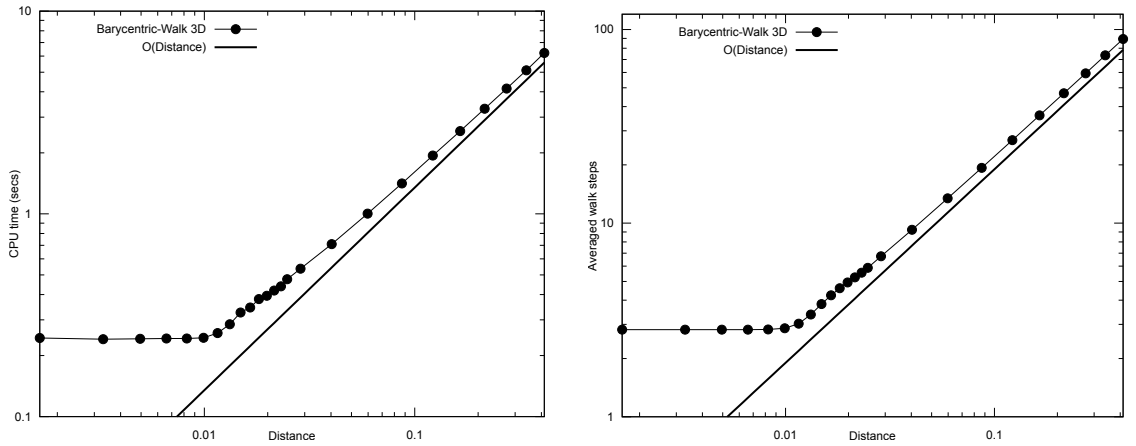
Figure 7: Execution times (left) and averaged walk steps (right) for the barycentric walk search on the whole mesh ( d = 3 , N \sim 4 \cdot 10^5 ), versus distance between start and end points, compared with the line of linear increase.
