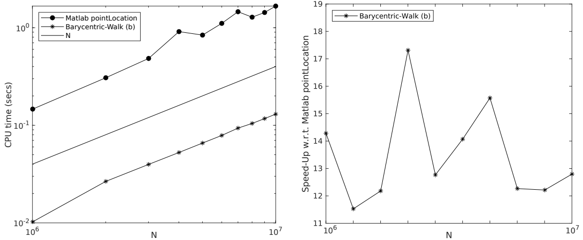
Figure 16: Search time (left) and improvement factor (right) of the barycentric walk with initialization strategy (BWb) versus the Matlab pointLocation , for 10^6 \lesssim N \lesssim 10^7 . Matlab pointLocation : black circles, strategy (BWb): crosses.
