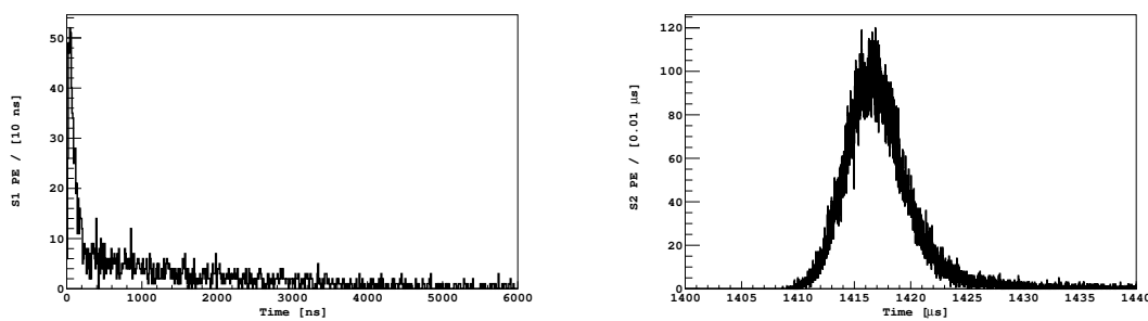
Fig. 75. Arrival time of S1 (Left) and S2 (Right) in DarkSide-20k, resulting from a complete simulation of the detector, electronics, and DAQ.
