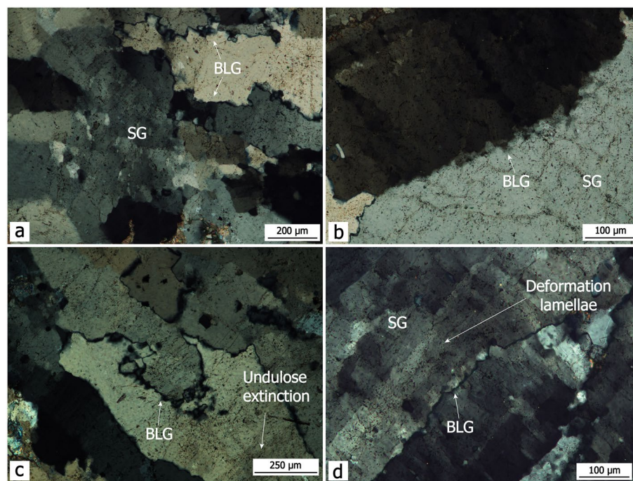
Figure 6. (a–d) Qz microfabric of sample S17-01 (Qz–Cb vein), showing evidence of ductile creep as indicated by sweeping undulose extinction, deformation lamellae and subgrain (SG) formation (crossed polars). Dynamic recrystallization textures are indicated by incipient bulging recrystallization (BLG).
