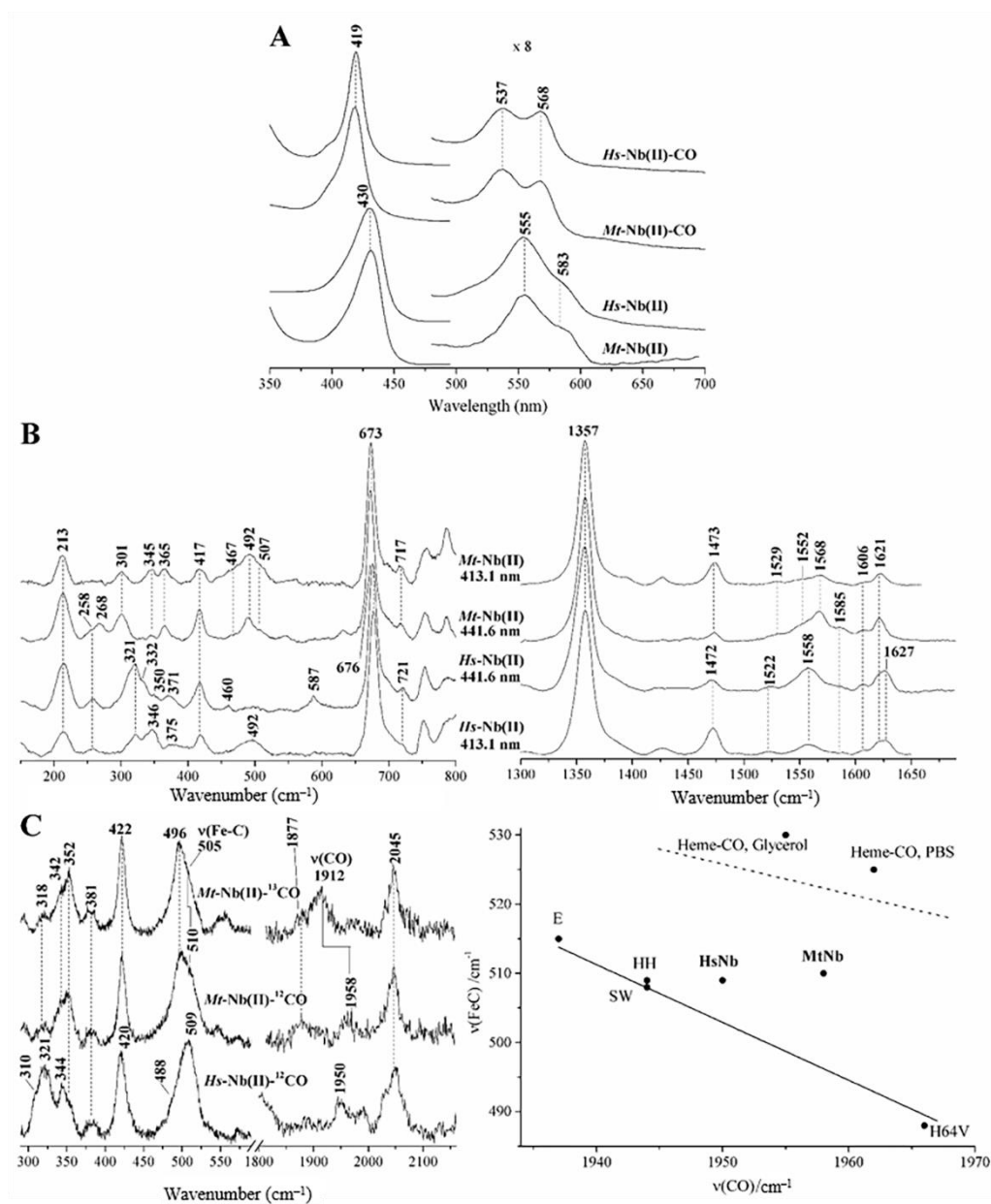
Figure 1. UV-Vis and RR spectra of Mt -Nb(II), Mt -Nb(II)-CO, Hs -Nb(II), and Hs -Nb(II)-CO. (A) UV-Vis spectra of Mt -Nb(II), Mt -Nb(II)-CO, Hs -Nb(II), and Hs -Nb(II)-CO at pH 6.0 and room temperature. (B) RR low frequency (left) and high frequency (right) spectra of Mt -Nb(II) (top) and Hs -Nb(II) (bottom) at pH 7.4 and room temperature with 413.1 and 441.6 nm excitation wavelength. Experimental conditions: 15 mW at the sample, 20 min integration time. (C) left: RR spectra of Mt -Nb(II)- ^{13}\text{C} O (top), Mt -Nb(II)- ^{12}\text{C} O (middle), and Hs -Nb(II)- ^{12}\text{C} O (bottom) in the 300–600 and 1800–2100 \text{cm}^{-1} regions (left and right, respectively), at pH 7.4 and room temperature with 413.1 excitation wavelength. Experimental conditions: 1 mW at the sample, 1 h (low-frequency region) or 2 h (high-frequency region) integration time. (C) right: Back-bonding correlation plot for the \nu(\text{Fe-C})/\nu(\text{CO}) stretching frequencies of the CO complexes of Mt -Nb and Hs -Nb together with heme-model compounds and representative Mbs, namely Pc -Mb, Cc -Mb, and the His64Val mutant of Pc -Mb (His64Val), at pH 7.4 and room temperature. The lower line represents six-coordinate carbonylated heme-proteins with imidazole as the sixth ligand; the upper line represents five-coordinate species, with no trans ligand, or six-coordinate carbonylated hemes with weak trans ligand.
