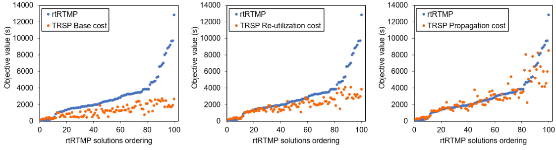
Figure 5: Correlation between TRSP (orange) and rtRTMP (blue) objective function values, when using Base, Re-utilization and Propagation costs
