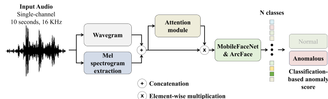
Fig. 1. Description of the proposed pipeline for USAD.
