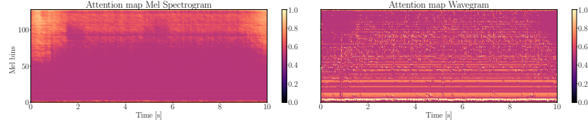
Fig. 3. Attention maps H = f_{\text{ATT}}(X) obtained from the attention module with acoustic features in Figure 2.
